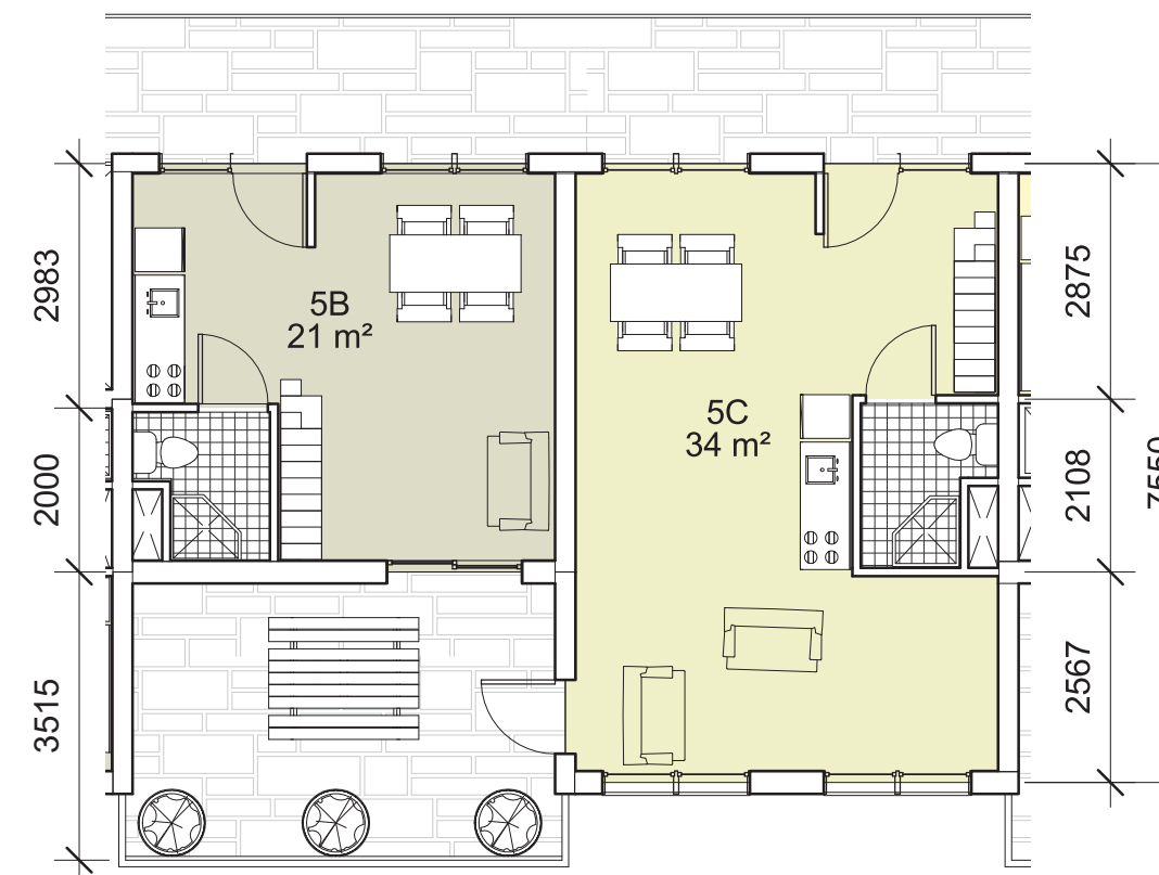
5th - Roof terrace and Gallery
