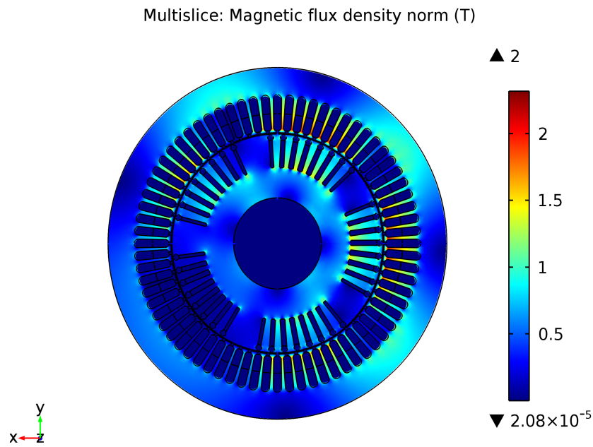
Figure 5.23: Plot of norm B from the non-linear model.
