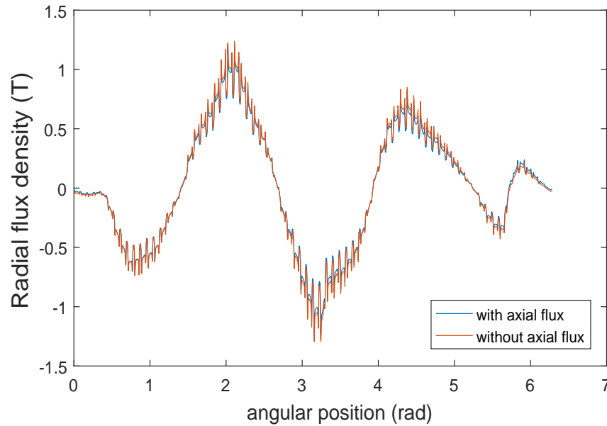
Figure 5.19: Comparison of radial flux densities at z = 239\text{mm} (right end), with and without axial flux contribution.
