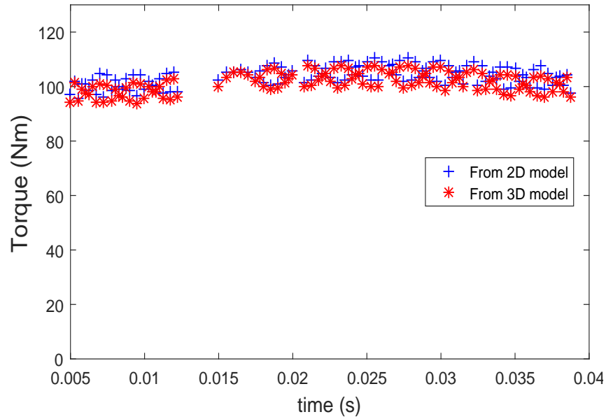
Figure 5.20: Comparison of torque values for non-skewed rotor.
