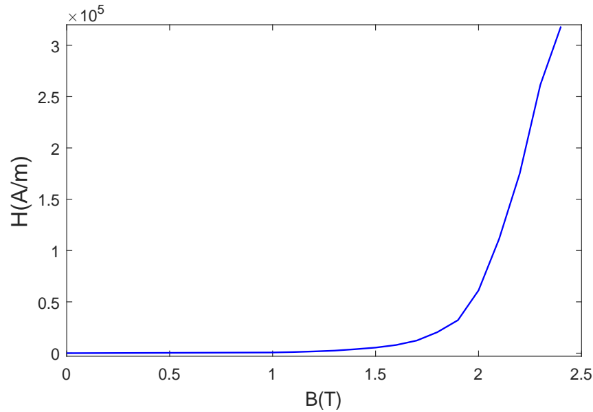
Figure 3.1: Typical HB curve for iron in machines
