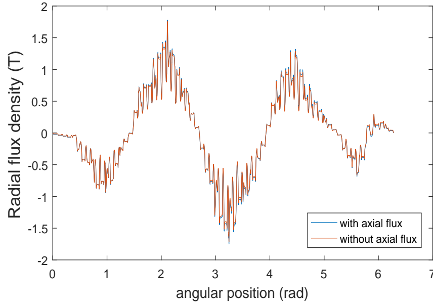
Figure 5.18: Comparison of radial flux densities at z = 1\text{mm} (left end), with and without axial flux contribution.
