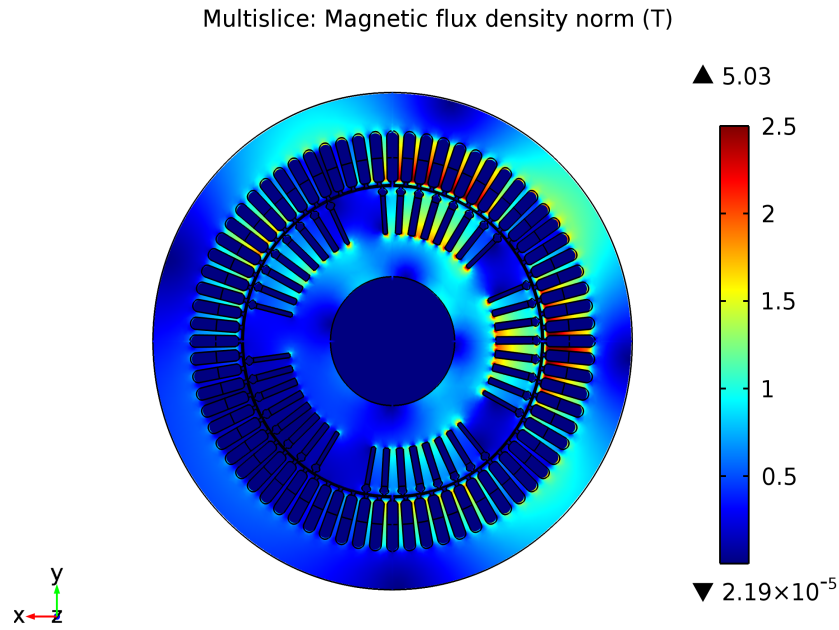
Figure 5.22: Plot of norm B from the linear model.
