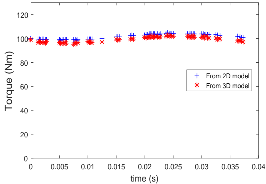
Figure 5.21: Comparison of torque values for rotor with 1 stator slot skew.
