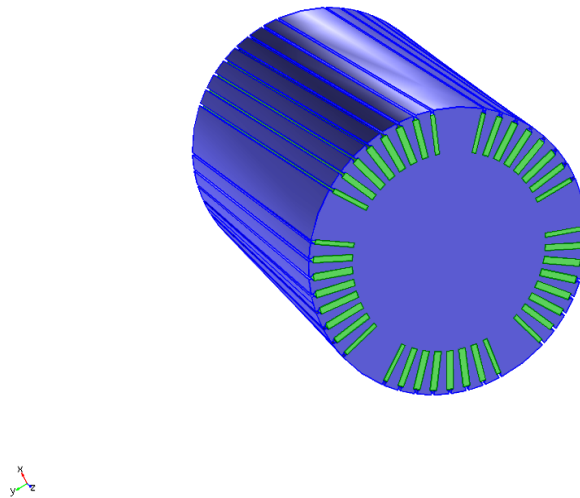
Figure 5.3: 3D BDFIM rotor geometry with skew.
