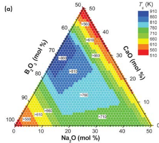
Fig. 4: T_g as a function of composition, from Meuro
