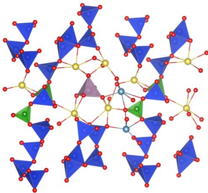
Fig. 5: Local structure of glass containing Mo, from Konstantinou
