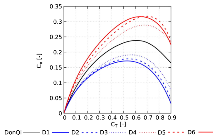
FIGURE 12 Effect of variable actuator disc (AD) loading on duct thrust force coefficient using disc Reynold-averaged Navier Stokes (RANS) solution [Colour figure can be viewed at wileyonlinelibrary.com ]
