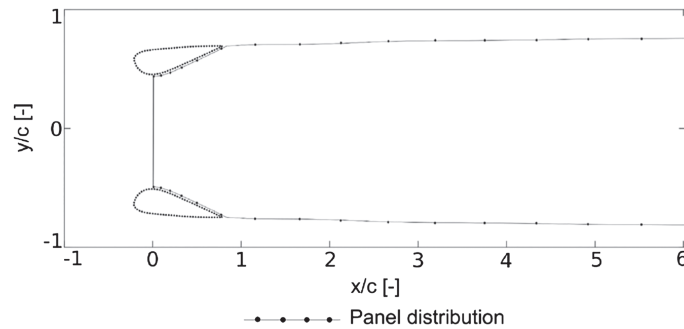
FIGURE 3 Panel distribution along the duct surface and the wake region used for the inviscid panel method calculations
