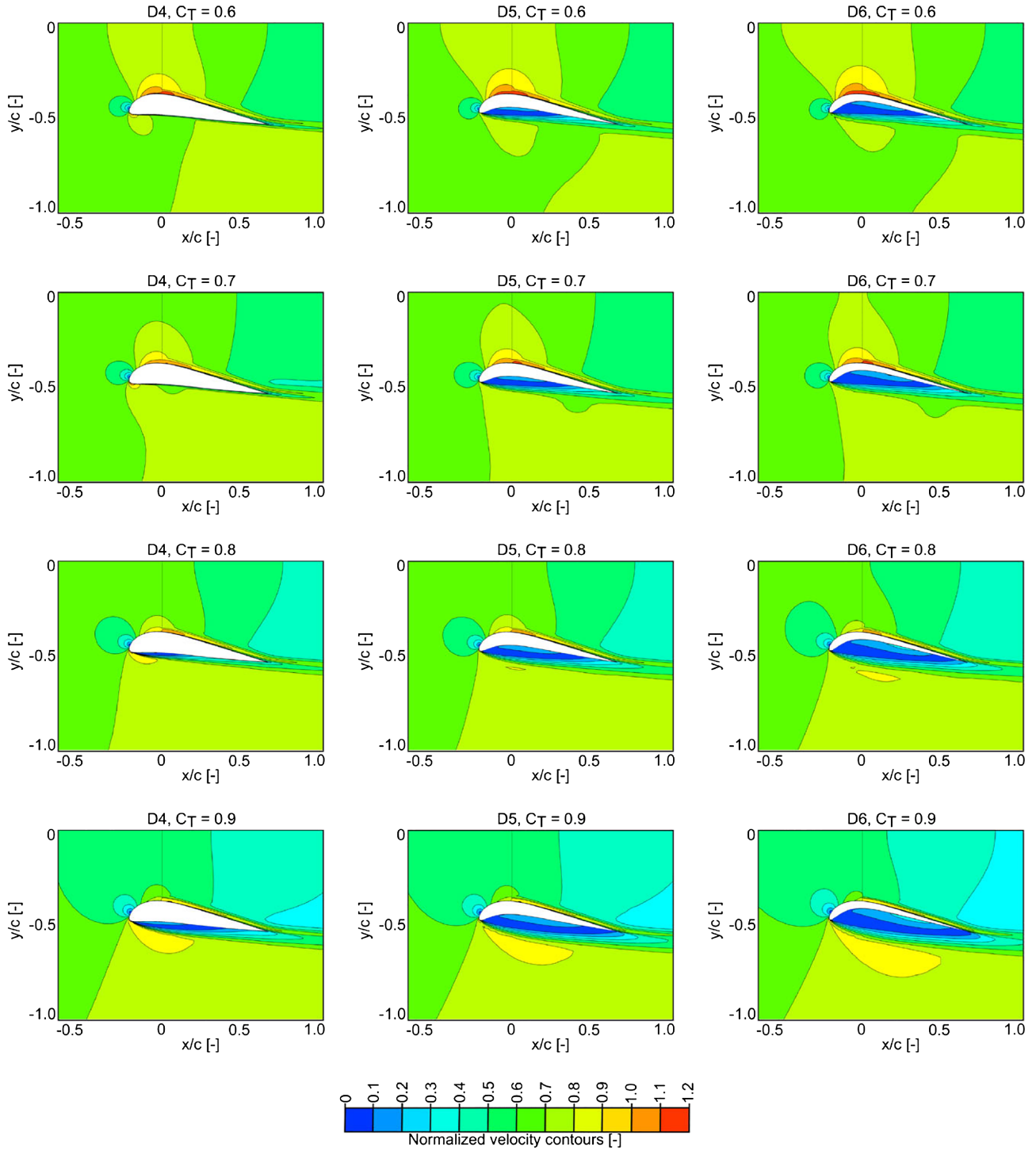
FIGURE 15 Velocity contours coloured with normalized streamwise velocity. The results are depicted for ducts D4, D5, and D6 (left to right) bearing C_T = 0.6, 0.7, 0.8 , and 0.9 (top to bottom) [Colour figure can be viewed at wileyonlinelibrary.com ]
