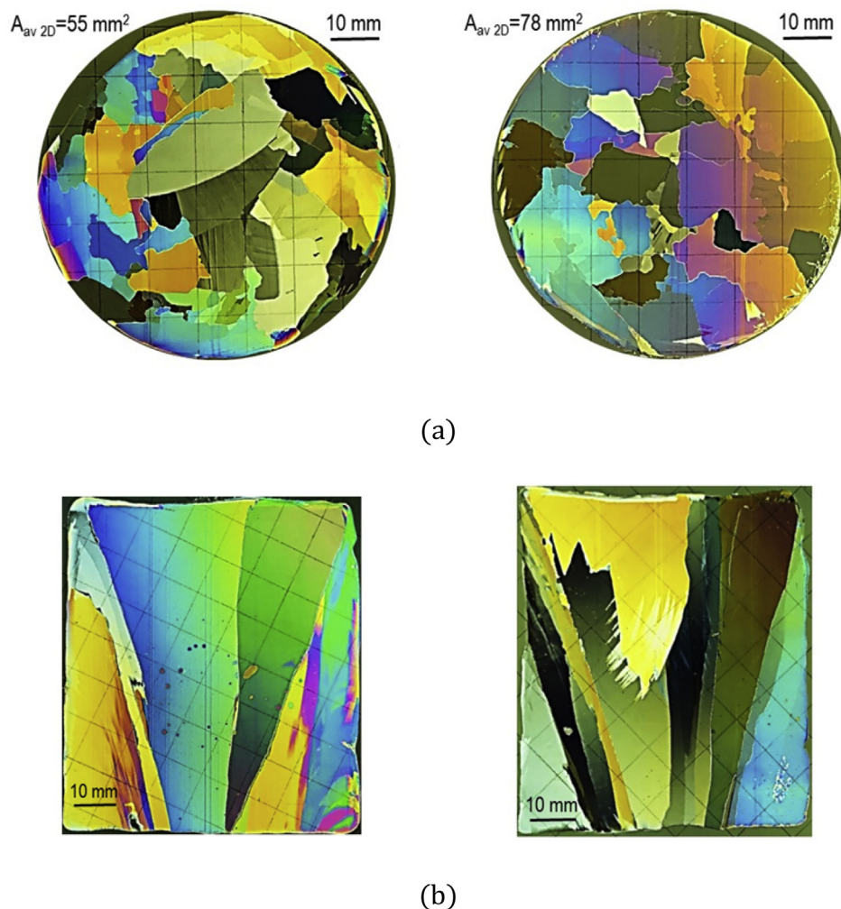
Fig. 5. Thin sections of typical ice samples (a) horizontal cross section (30 mm above the contact with concrete); (b) vertical cross section (contact line at the top).
