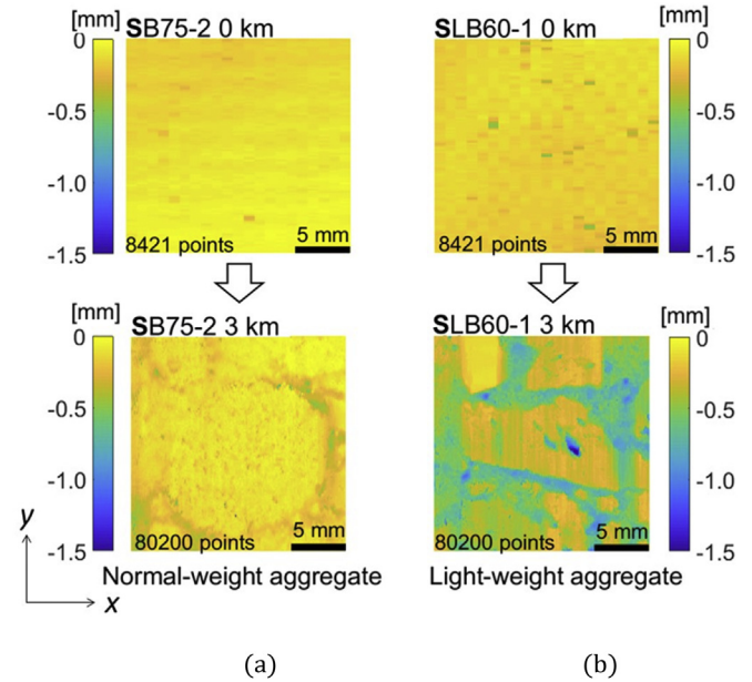
Fig. 13. Parts of the surface scan before and after 3 km testing: (a) normal-weight aggregate; (b) light-weight aggregate. (Note: the resolution for scans before the test was lower than for scans after the test.)
