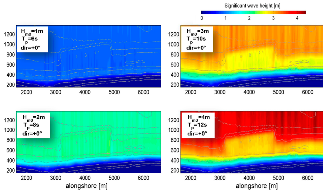
Figure 11. Modelled wave transformation for four shore-normal wave height classes at the Ter Heijde'97 shoreface nourishment using the XBeach model (using January 1998 bathymetry survey).
