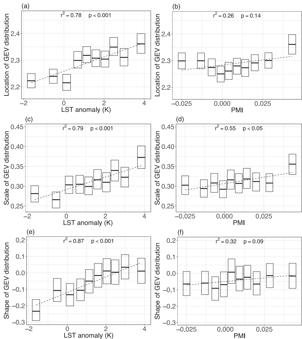
Fig. 5. Location, scale and shape of the GEV distribution of log-transformed fire duration in decile bins of LST anomaly and PMI.
