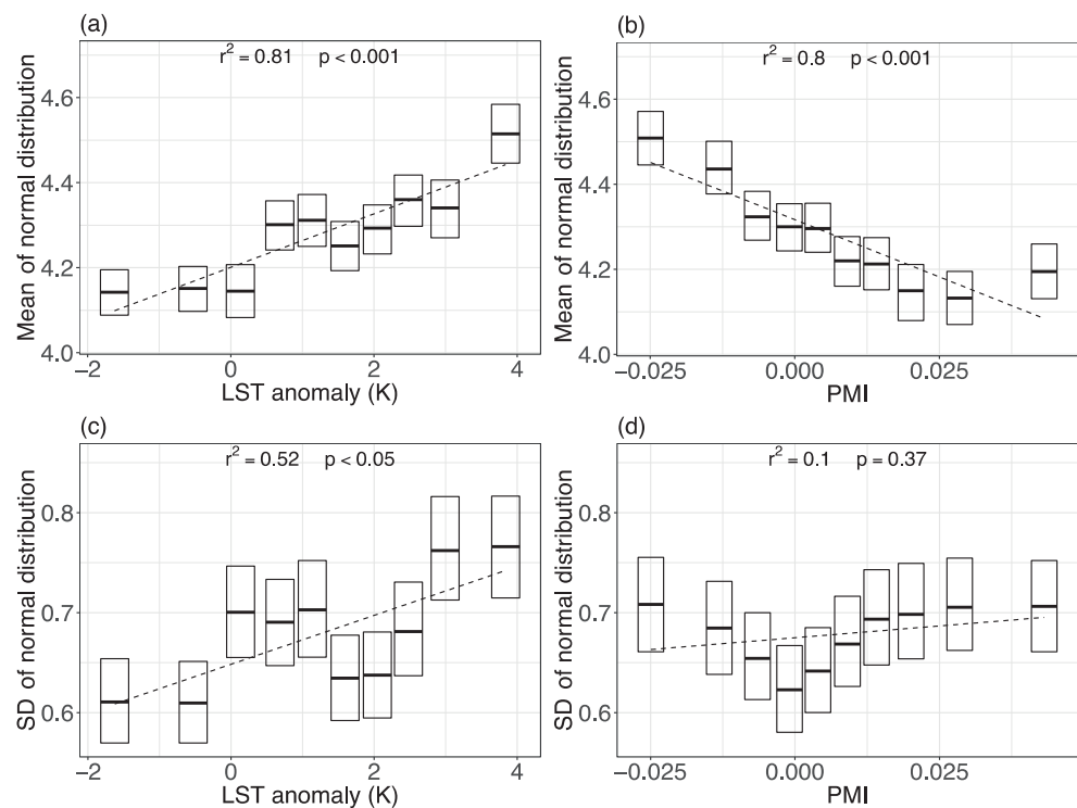
Fig. 4. Mean and standard deviation of normal distribution of log-transformed burned area in decile bins of LST anomaly and PMI.
