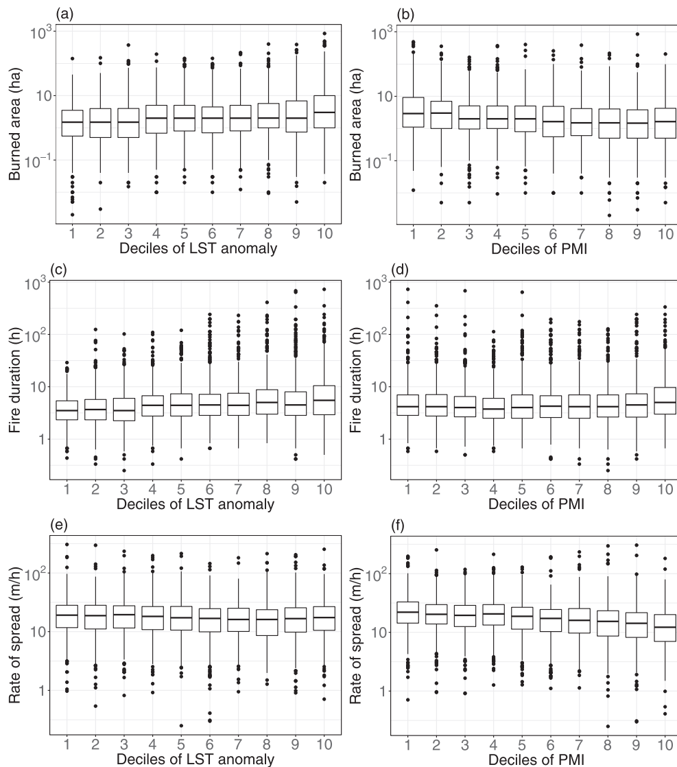
Fig. 3. Boxplots of burned area, fire duration and rate of spread in decile bins of LST anomaly and PMI.
