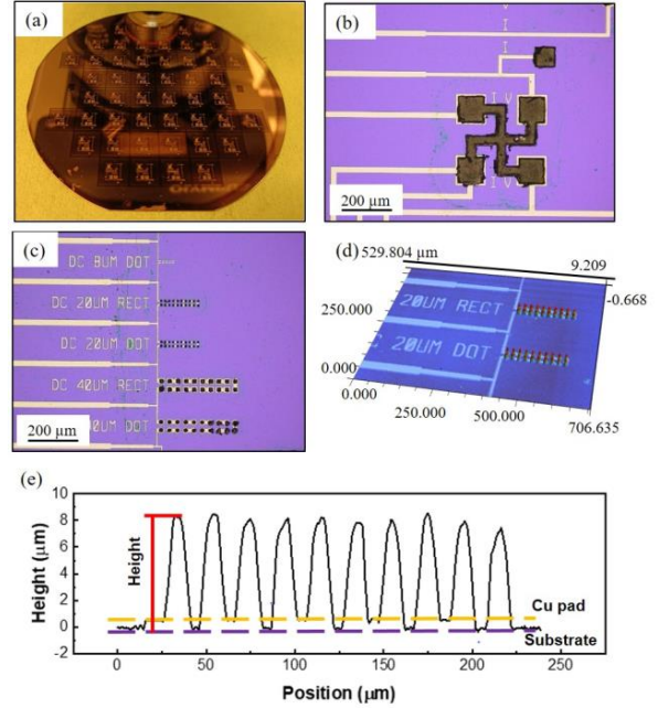
Fig. 3. Test bottom pattern obtained after LSP process. (a) Wafer-scale nano-Cu pattern shown in the dark non-reflected area, (b) Greek cross nano-Cu pattern used for sheet resistance measurements, (c) and (d) representing the resulting 2D and 3D information, and (e) surface profile of the nano-Cu bumps.
