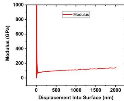
Fig. 11. The elastic modulus of sintered Cu from the surface to a depth of 2 \mu\text{m} .
