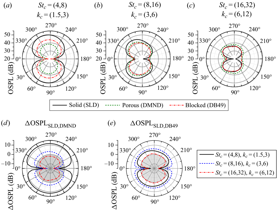
Figure 10. Far-field noise directivity of solid, porous and blocked TE, plotted in terms of overall sound pressure level (OSPL) integrated over three different frequency ranges: (a) 4 < St_c < 8 , (b) 8 < St_c < 16 and (c) 16 < St_c < 32 . The OSPL difference between the solid and the porous and blocked TE cases is plotted in panels (d) and (e); the grey circle at the centre of the polar plot indicates regions of noise increase. The aerofoil leading edge is facing towards 0^\circ .
