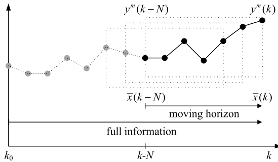
Figure 4.7 Parameter estimation with MHE scheme (adapted from [23]).
