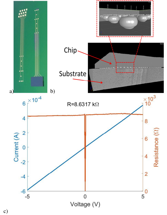
Fig. 10. Preliminary results after bonding. CT scans and 2-point measurements have been performed to ensure that the bonding process was successful.
