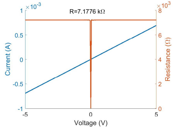
Fig. 11. 2-point measurement results for dummy chips bonded on a graphene substrate using a conductive adhesive (CA) flip-chip bonding technique.
