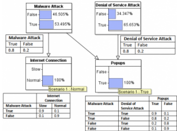
Fig. 1. Standard BN Model - Example
