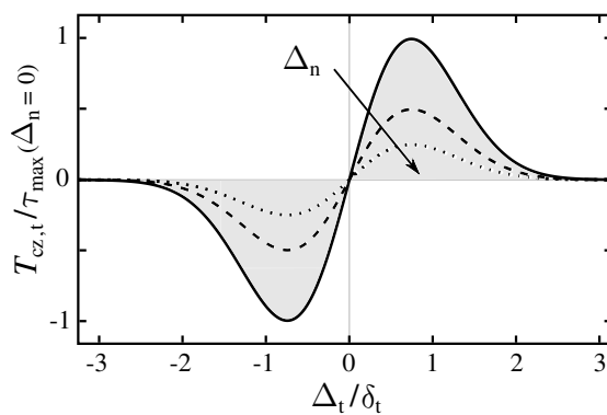
(b) tangential traction
