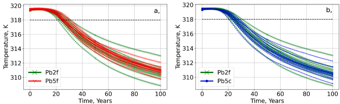
Fig. 14. Comparison plot of production temperatures for the process-based scenarios. a, comparing Pb2f (green curves) to Pb5f (red curves); b, comparing Pb2f (green curves) to Pb5c (blue curves). Black dashed lines highlight the temperature at which we designate breakthrough to occur.
