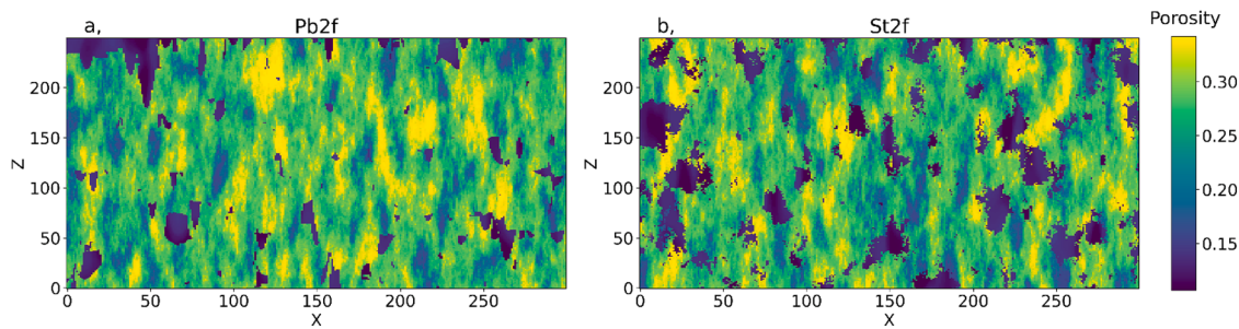
Fig. 7. Example plot of porosity cross-sections along the x-axis of the reservoir domain from a, Pb2f and b, St2f. Axes show number of cells and z-axis is exaggerated 5 times for readability.
