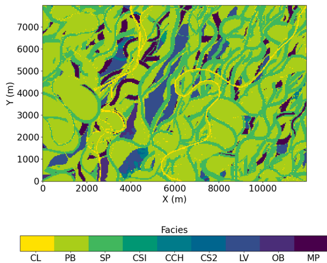
Fig. 3. Example of a single process-based realization showing the 9 different facies; Channel lag (CL), Point bar (PB), Sand plug (SP), Crevasse splay type 1 (CSI), Crevasse channels (CCH), Crevasse splay type 2 (CS2), Levee (LV), Overbank (OB) and Mud plug (MP).
