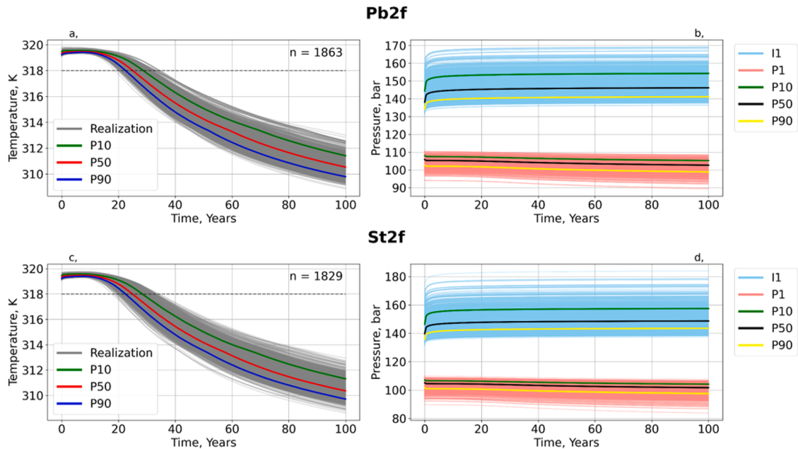
Fig. 9. Production temperature and pressure for all process-based (a, b) and stochastic realizations (c, d) in Pb2f and St2f, respectively. The dashed grey line represents the point of thermal breakthrough, considered as a temperature drop of 1 K from the initial production temperature.
