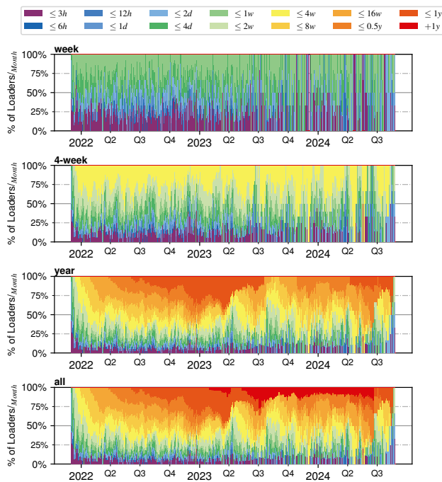
Figure 9: Malware storage activity days over time.
