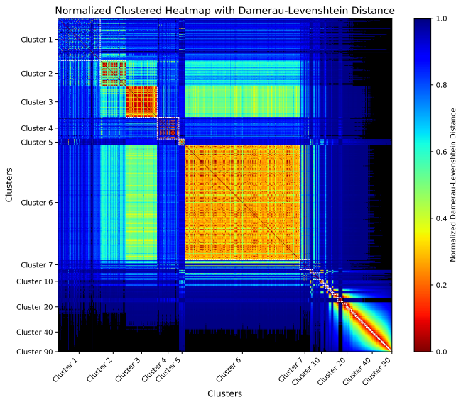
Figure 5: Normalized DLD Matrix.
