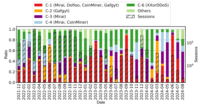
Figure 6: Top 5 clusters (bots) over time.
