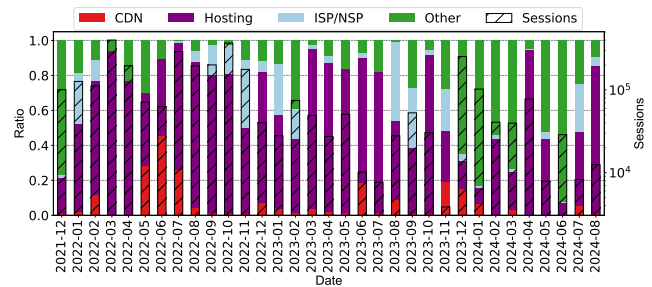
Figure 17: AS Types of Malware storage location seen over time.
