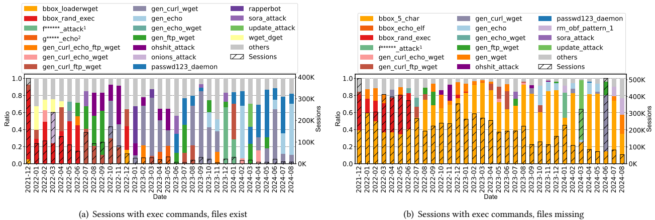
Figure 4: Sessions that attempt to execute files.
