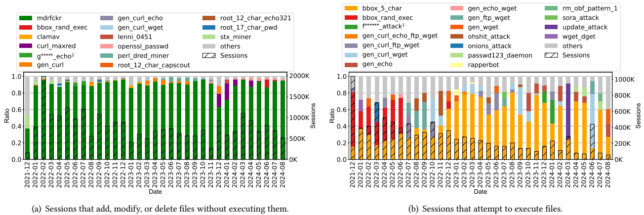
Figure 3: Sessions that change the initial state of the honeypot.
