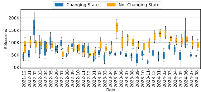
Figure 1: Sessions that contain commands split in two categories. In blue, we have the sessions that change the state of the honeypot and in orange otherwise.
