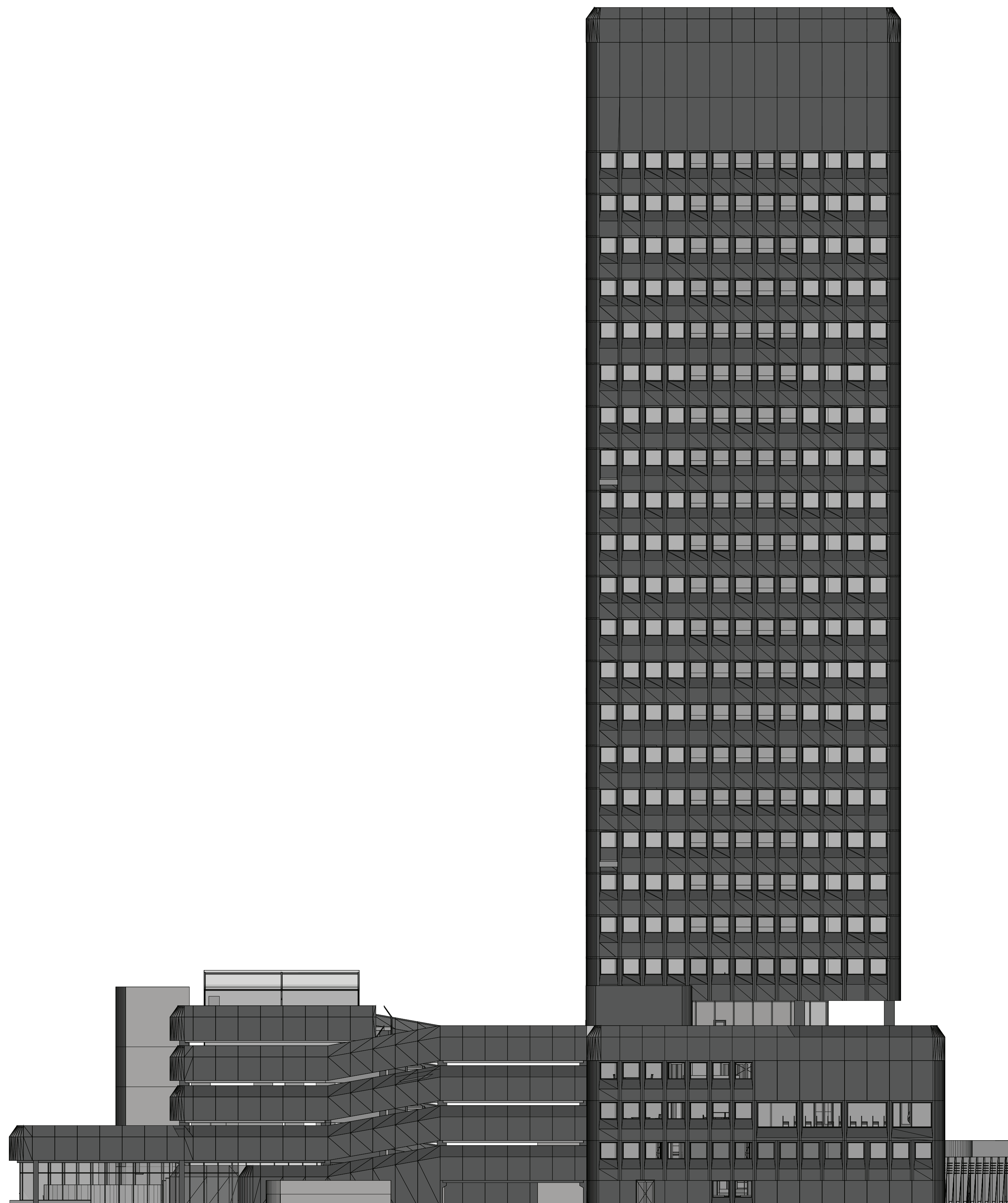
Elevation - North 1:200
