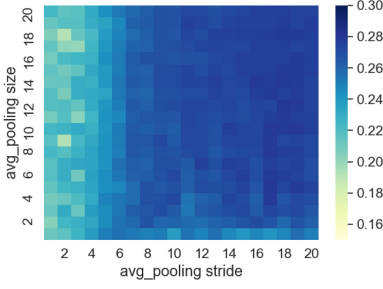
(a) ACC : tuning the first average-pooling layer (min: 0.192; max: 0.280)
