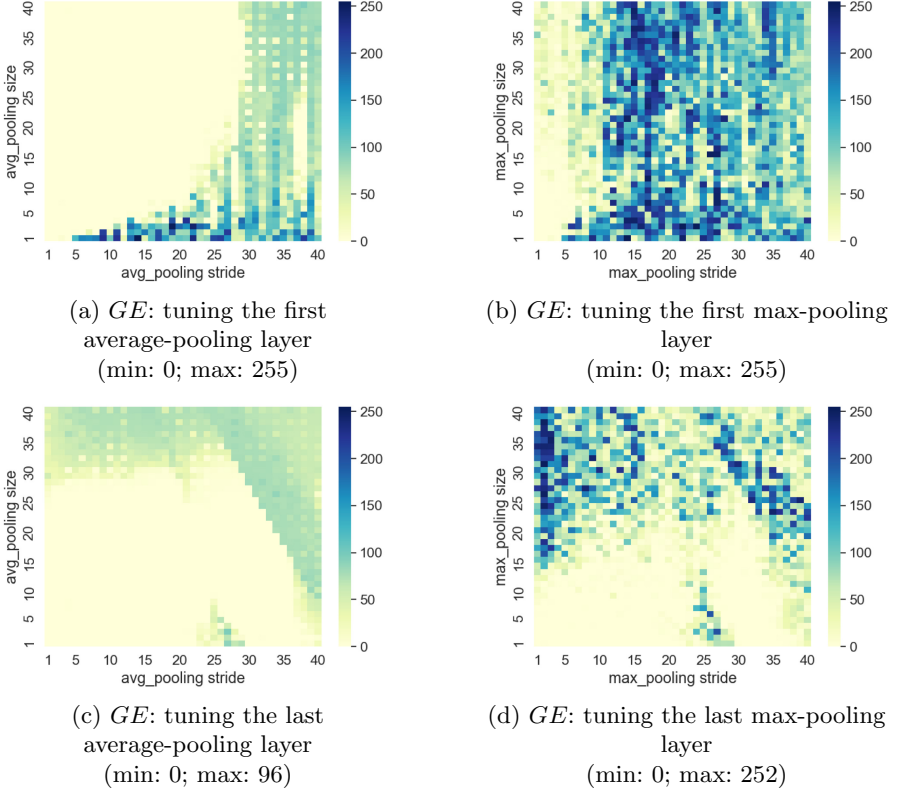
Fig. 8. GE for standardized dataset with average-/max-pooling layer for the HW leakage model on ASCAD r .
