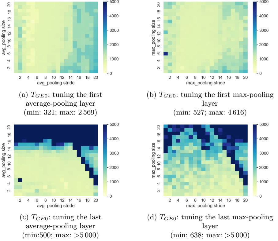
Fig. 6. T_{GE0} for the standardized dataset with average-/max-pooling layer for the HW leakage model on ASCAD.f.
