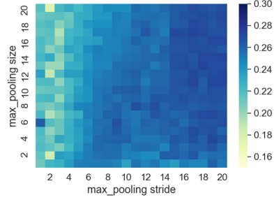
(b) ACC : tuning the first max-pooling layer (min: 0.176; max: 0.274)
