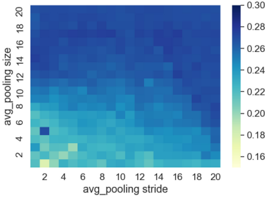
(c) ACC : tuning the last average-pooling layer (min: 0.177; max: 0.277)
