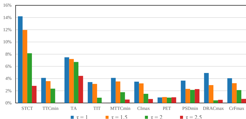
Figure 6. Surrogate safety indicators and the percentage of SSI accidents for vehicle and bike interaction (Benchmark Experiment).
