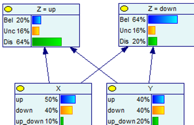
Fig. 8. Calculating the epistemic uncertainty of Z = \{\text{up}\} and Z = \{\text{down}\} without additional nodes of Bel and Pls functions.
