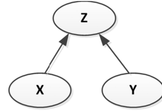
Fig. 5. A typical Bayesian network.
