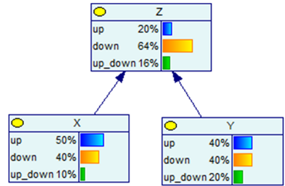
Fig. 6. EN for uncertainty assessment using BN inference algorithm.
