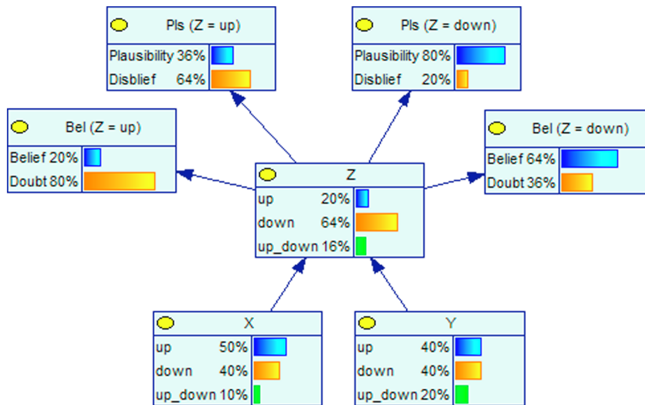
Fig. 7. Calculating the interval probabilities of Z = \{\text{up}\} and Z = \{\text{down}\} using Bel and Pls nodes.
