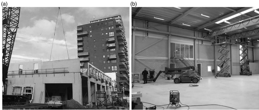
Figure 1. (a) Under-construction housing tower building project of case B on the left, and (b) the interior of utility building of case C on the right.
