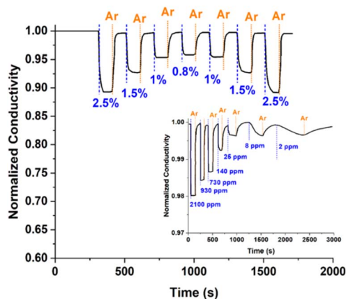
Fig. 3 Changes in the conductivity of the Pd NP-based films upon cycling the concentration of \text{H}_2 in the overlaying gas from 0.8 to 2.5%. Inset: Changes in the conductivity of the films when the concentration of \text{H}_2 was cycle-reduced from 2100 to 2 ppm. The dashed blue lines indicate the times when the films were exploded to \text{H}_2 , while the dotted orange lines mark the introduction of Ar in the sensing set-up.
