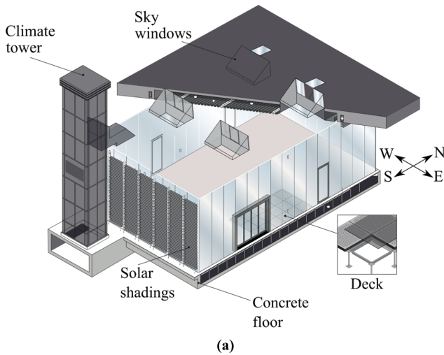
Fig. 1. Building configuration with glazed facades, dynamic solar shades, deck and concrete floor, sky windows, and climate tower.
