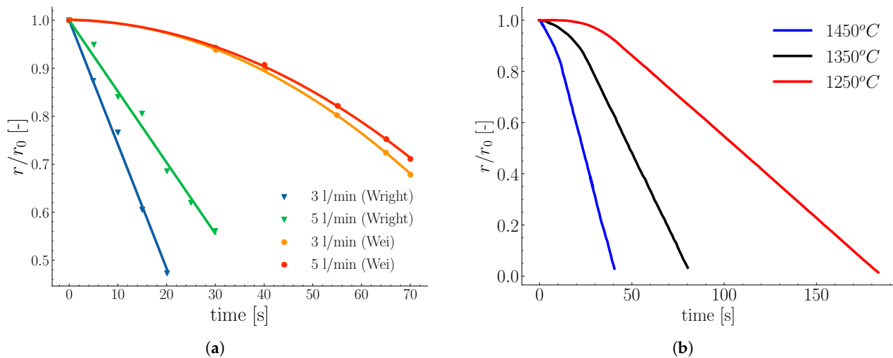
Figure 6. Melting rods with different stirring modes; (a) rod specification: radius r_0 = 6 mm, composition: C = 0.26\% , Mn = 0.7\% , bath specification T = 1400\text{ °C} , C = 4.5\% , and stirring gas is nitrogen [12]. Wei's rod specification: initial radii ( r_0 ) are 10 and 25 mm, composition: C = 0.45\% , Mn = 0.5\% , and molten bath temperature T = 1400\text{ °C} and C = 3.1\% [62]; (b) dimensionless melting profile of rotating (923 rpm) carbon steel rod (radius r_0 = 20 mm) immersed in liquid Fe-C at different molten bath temperatures [49].
