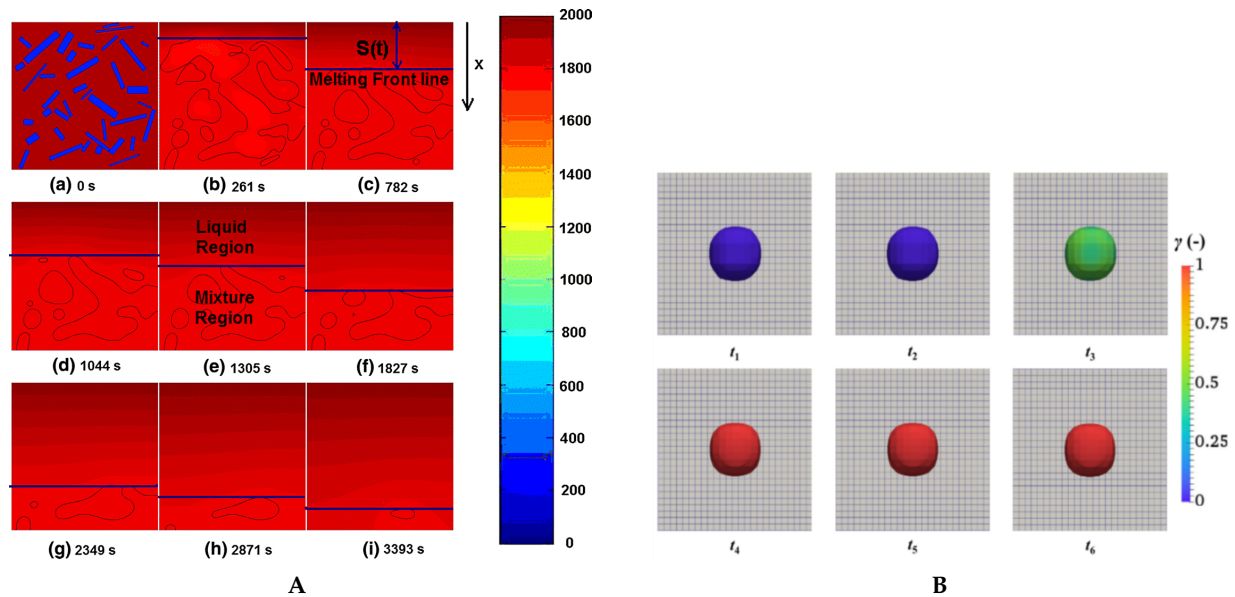
Figure 7. (A) Modeling melting of randomly distributed scrap using phase-field method colored by temperature (adapted from [6], Copyright 2008 Springer Nature. The Minerals, Metals & Materials Society and ASM International . Used with permission). (B) Time evolution of \text{Fe}_x\text{C}_y particles using (VOF); particles are colored by volume fraction (1 for liquid and 0 for solid) (adapted from [84], copyright 2023, with kind permission from Elsevier).
