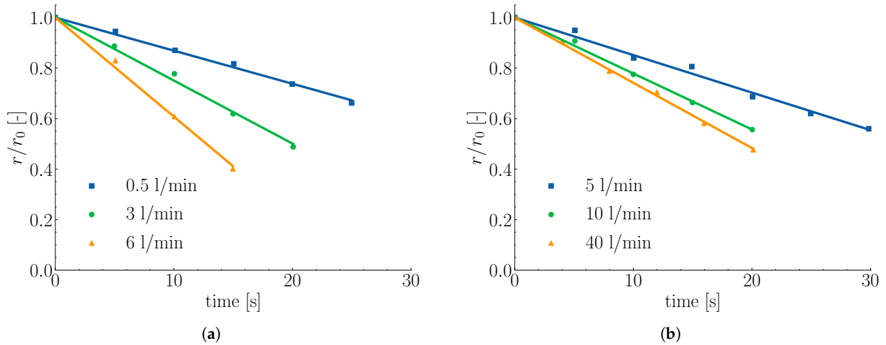
Figure 5. Dissolution of 6 mm radius steel rods (composition: C = 0.26\% , Mn = 0.7\% , at bath temperature T = 1400\text{ °C} , and carbon concentration C = 4.5\% ) at different nitrogen gas flow rates in (a) 1 kg iron bath and (b) 25 kg iron bath [12].
