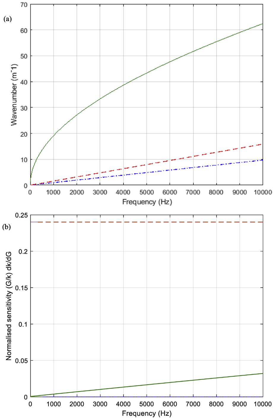
Fig. 7. Foam-cored panel: (a) wavenumbers and (b) normalised sensitivity of wavenumbers with respect to shear modulus of the core: — bending, --- shear and -.- axial dominated waves.
