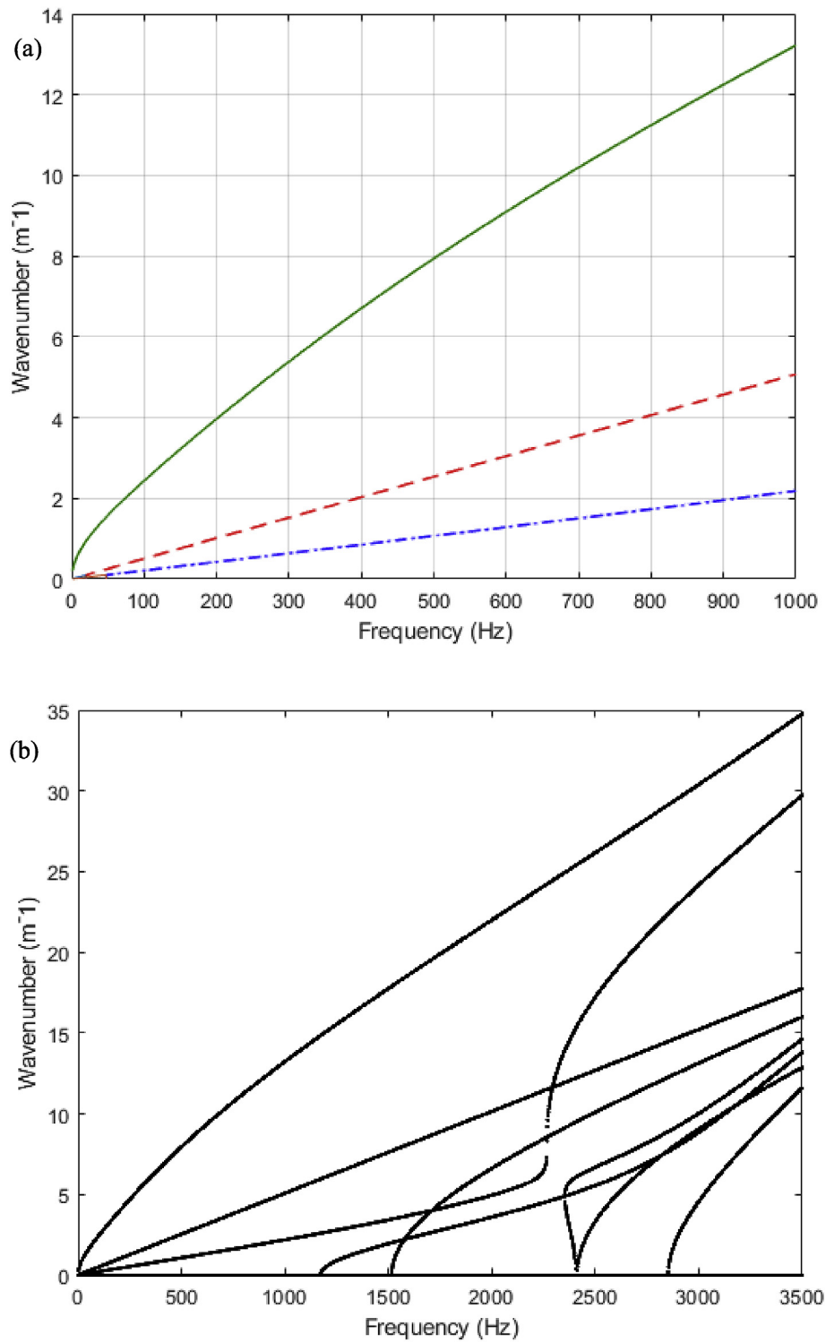
Fig. 9. Wavenumbers for CLT panel: (a) lower frequencies — bending, --- shear and -.- axial dominated waves, and (b) higher frequencies.
