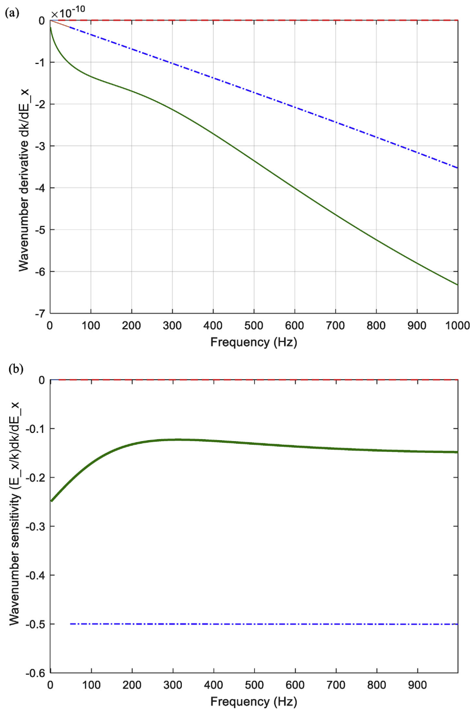
Fig. 10. CLT panel: (a) sensitivity and (b) normalised sensitivity of wavenumbers with respect to elastic modulus along-grain, lower frequencies: — bending, --- shear and -.- axial dominated waves.
