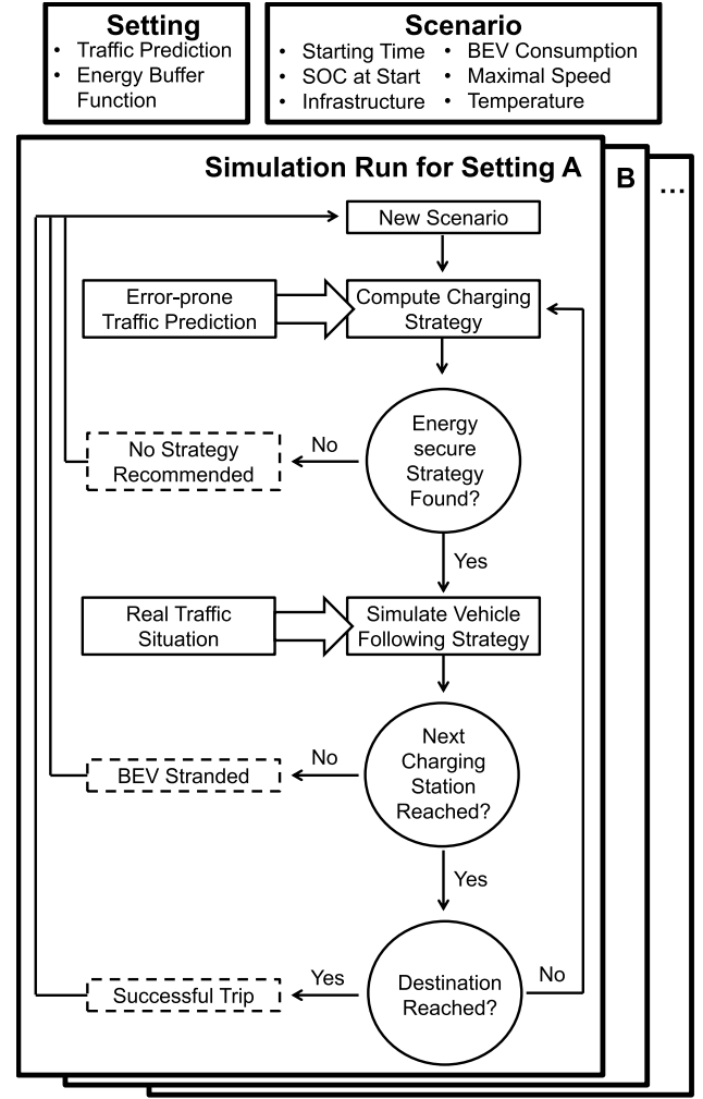
Fig. 5. Structure of simulation study.
