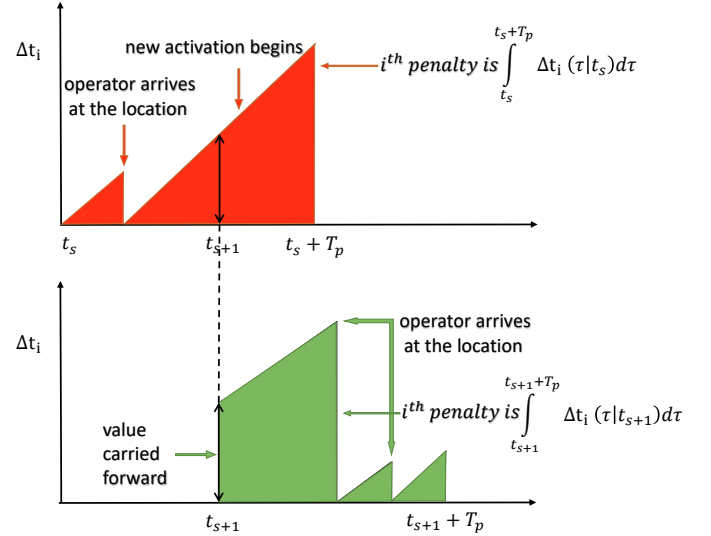
Figure 1. Definition of the variables \Delta t_i(\tau|t) . The i^{\text{th}} component of the penalty J_{\text{loc}}(t_s) ( t_{s+1} ), respectively) represents the red (green, respectively) area shown.
