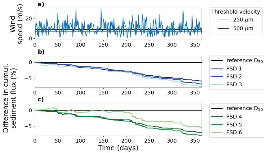
Figure 5.10: (a) 1-year variable wind scenario. The horizontal lines in the wind plot indicate the threshold velocity for the single-fraction case of 250 \mu\text{m} (grey) and 500 \mu\text{m} (black). (b) and (c) Cumulative sediment flux of each tested particle size distribution (PSD) as shown in Figure 5.3e, compared to the reference case (black). For each PSD, the reference case corresponds to the median grain size of the PSD. The blue colors in (b) have a median grain size of around 250 \mu\text{m} , the green colors in (c) have a median grain size around 500 \mu\text{m} .
