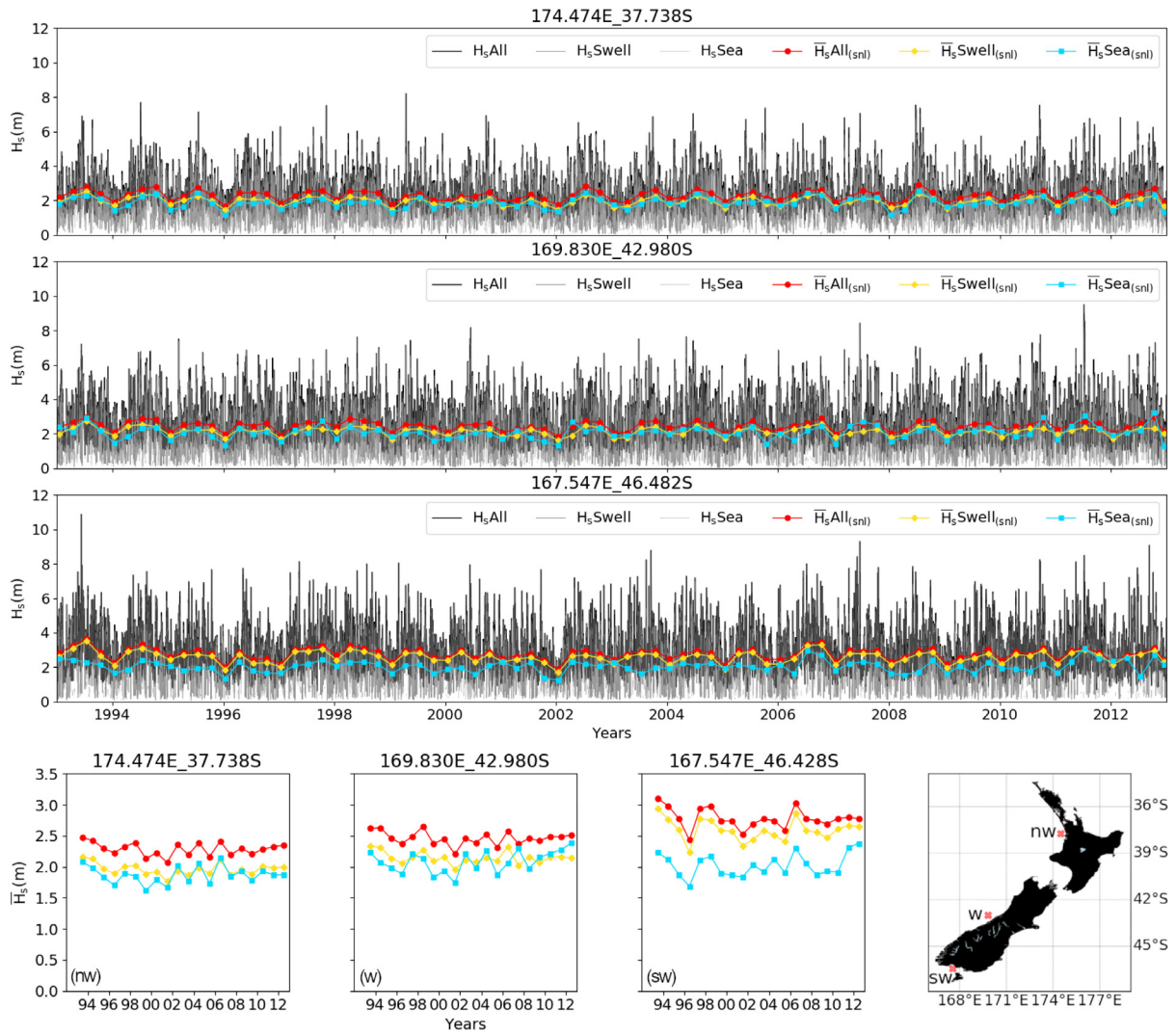
Fig. 8. Wave height timeseries of the three different locations along the west coast of New Zealand: points nw (174.474°E, 37.738°S, first row), w (169.830°E, 42.980°S, second row) and sw (167.547°E, 46.428°S, third row). Lines plotted in black, darkgrey and lightgrey show the 3-hourly total, wind-sea, and swell wave heights respectively. Red lines with circles, yellow lines with diamonds and light blue lines with squares show the seasonal (DJF, MAM, JJA, SON — first to third row plots) and yearly (fourth row, first to third columns) mean wave heights of integrated, swell and wind-sea waves. Geographic location of each point is shown in the bottom right map.
