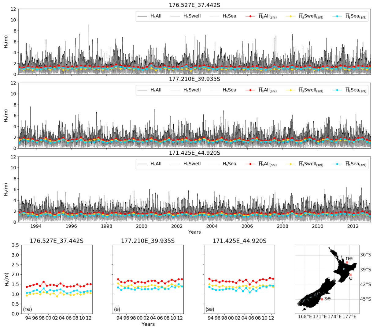
Fig. 9. Same as Fig. 8 but for three different locations off the east coast, as displayed in the bottom map. Points are: ne (176.527°E, 37.442°S), e (177.210°E, 39.935°S) and se (171.42°E, 44.920°S).
