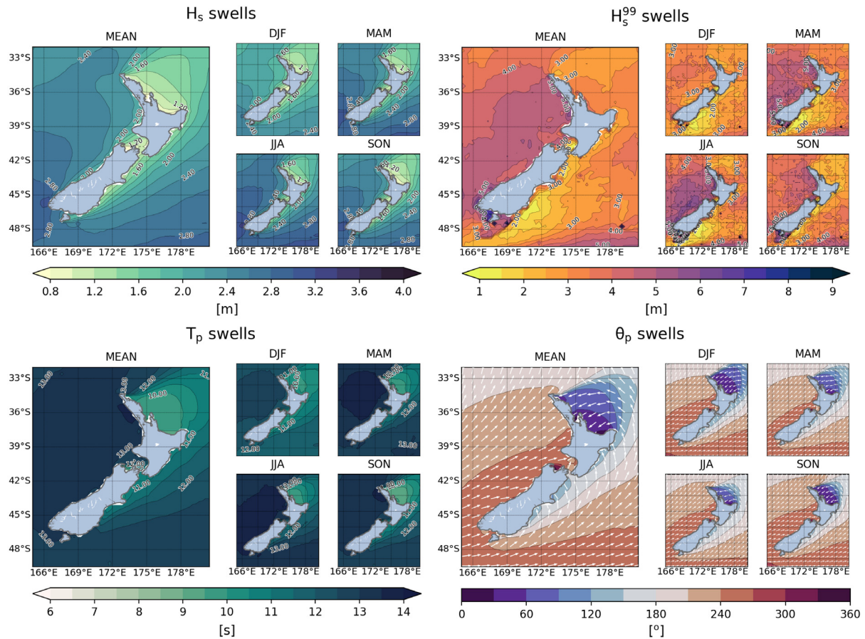
Fig. 5. Same as Fig. 4 but for aggregated swells.
