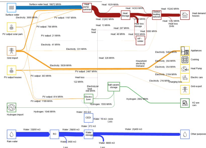
Figure 10. Sankey diagram of the yearly energy and water flows in the power-to-X system. An extra flow is added to the Sankey diagram to show the heat production, storage, and houses' heat demand when a low-temperature district heating system is installed in the neighborhood. The electricity demand of the houses is reduced compared to the other scenarios, as only 354 MWh of electricity is used by the booster heat pumps for tap water production. The district heating network makes a fuel cell for demand peak shaving redundant. The heat pump is shown twice in the Sankey diagram, although only one large-scale heat pump is installed. This large-scale heat pump is used in summer to produce heat (Heat pump summer) and partly in winter as well (HP-winter) to increase the temperature of the heat storage system to a sufficient temperature.
