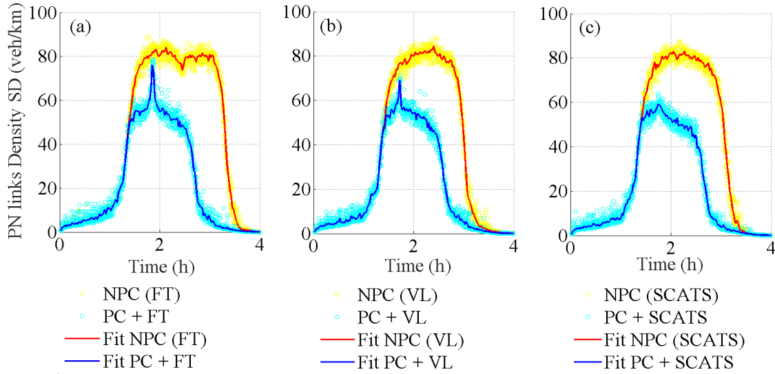
Figure 10 PN link density SD vs. time for (a) NPC (FT) and PC + FT; (b) NPC (VL) and PC + VL; (c) NPC (SCATS) and PC + SCATS
