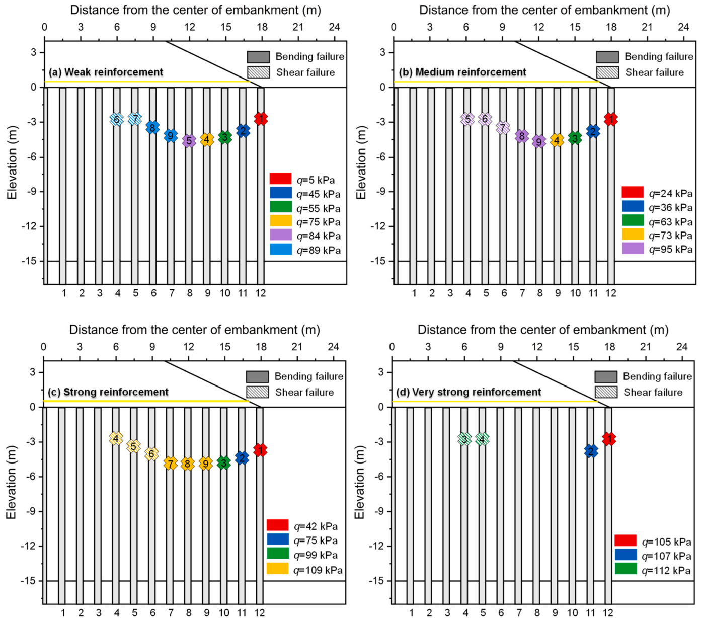
Fig. 21. Influence of tensile stiffness on the column failure loads and sequences of GRCS embankments: (a) weak reinforcement; (b) medium reinforcement; (c) strong reinforcement and (d) very strong reinforcement.
