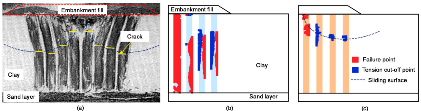
Fig. 8. Development of plastic failure zone: (a) Centrifuge test (form [15]); (b) MC model; (c) Concrete model.
