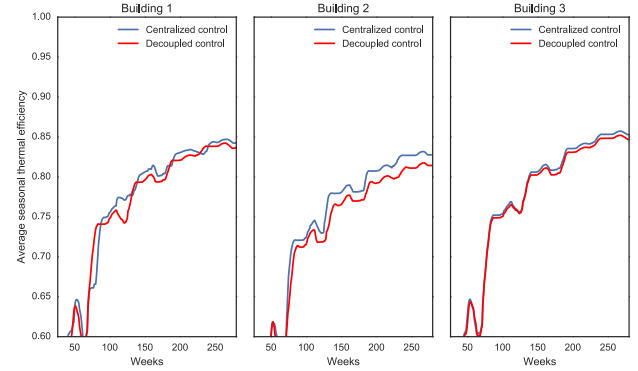
Fig. 4. Impact of DS and CS on average thermal efficiency.
