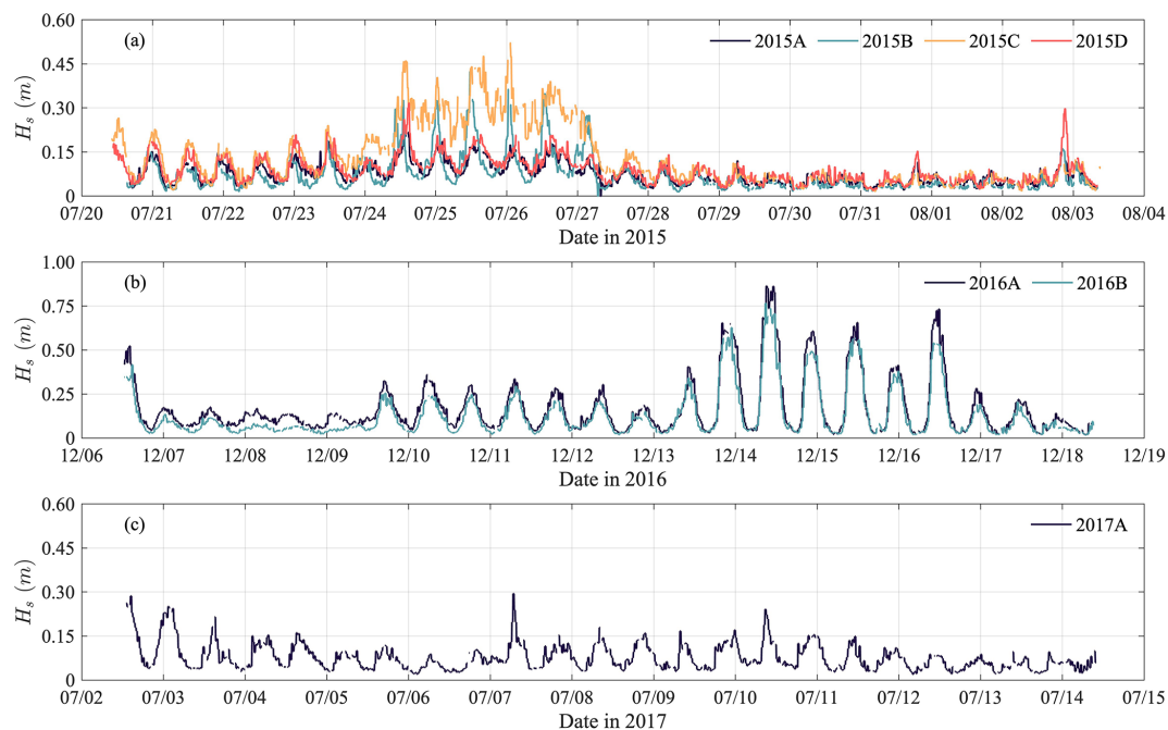
Figure 5. Significant wave heights recorded by RBRs in 2015, 2016, and 2017.
