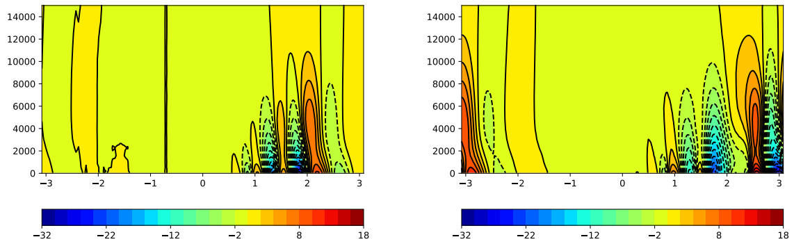
Figure 6: Baroclinic instability test case: Zonal-vertical pressure slice at 50^\circ N , days 8 and 10.
