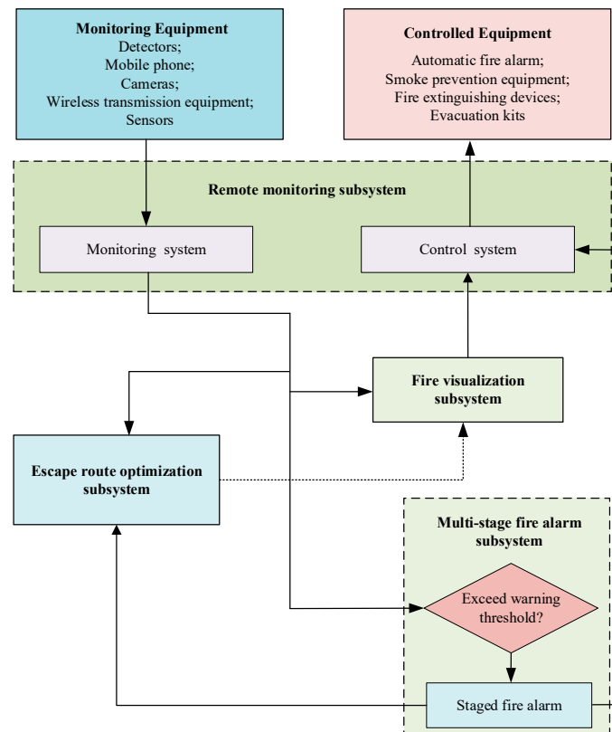
Figure 2. Operation process of the BIM-based fire safety management system.
