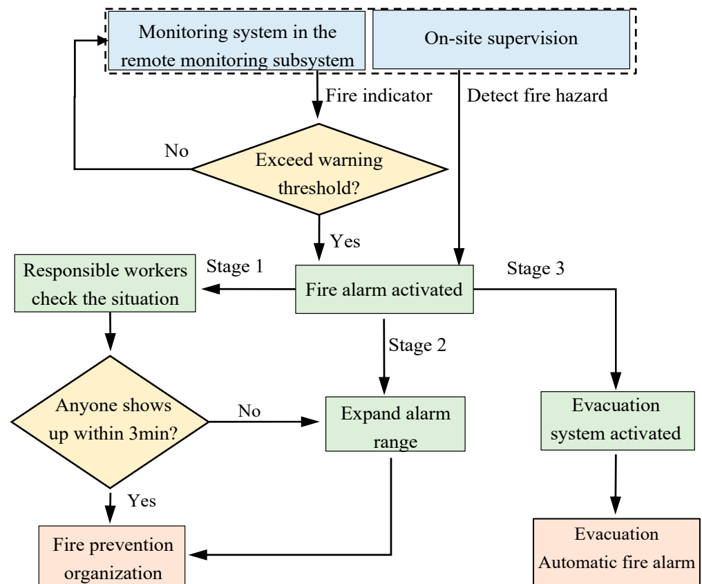
Figure 6. Schematic of the multi-stage fire alarm subsystem.
