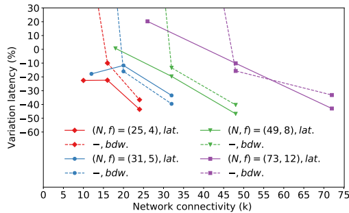
Fig. 10. Latency improvement over BDOpt - 16B payload.
