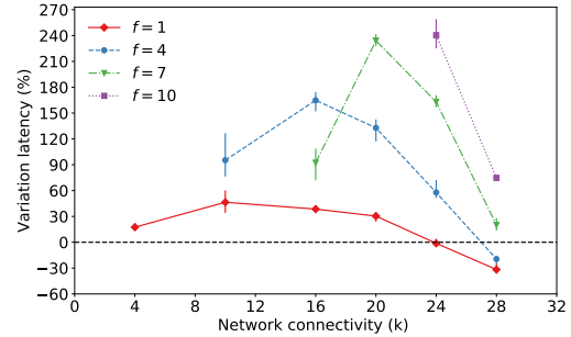
Fig. 5. MBD.11’s latency impact - N = 31 , 16KB payload.
