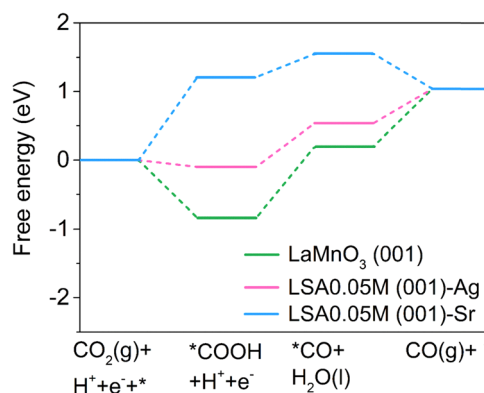
FIGURE 5 The calculated free energy for ECR to CO on \text{LaMnO}_3 (001), LSA0.05M (001)-Ag surface, and LSA0.05M (001)-Sr surface. LSA0.05M, (\text{La}_{0.8}\text{Sr}_{0.2})_{0.95}\text{Ag}_{0.05}\text{MnO}_{3-\delta} .
