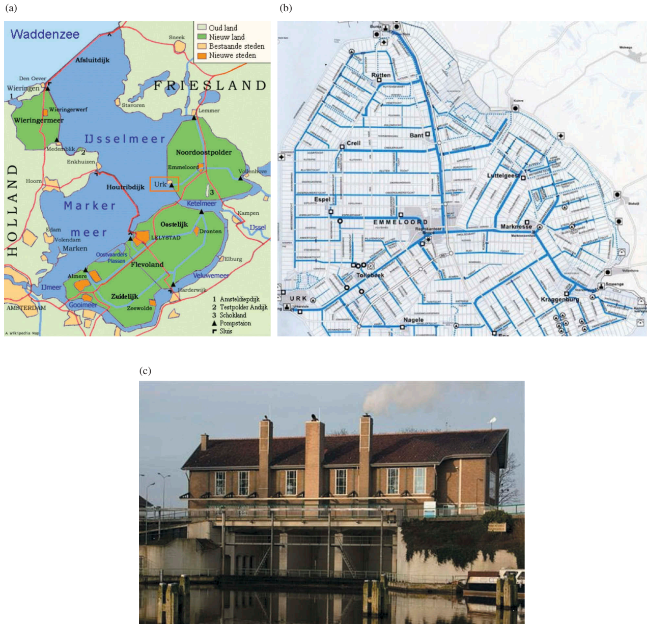
Figure 2. Maps of the Zuyder sea works (a) (Delta Works Online Foundation, 2004. Published with permission) and the Noordoostpolder (b) (Waterschap Zuiderzeeland, 2004. Published with permission) and a picture of pumping station Vissering (c) (Waterschap Zuiderzeeland, 2018. Published with permission.). The red arrow indicates the location of the pumping station.
