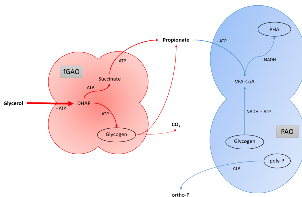
Fig. 7. Graphical representation of anaerobic glycerol conversion by aerobic granular sludge. DHAP: dihydroxyacetone phosphate, PHA: polyhydroxyalkanoates, Poly-P: polyphosphate, VFA-CoA: the combination of acetyl and propionyl-CoA.
