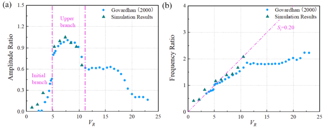
Fig. 4. Amplitude and frequency variation with reduced velocity for a low-mass-damping cylinder. S_t is Strouhal number.
