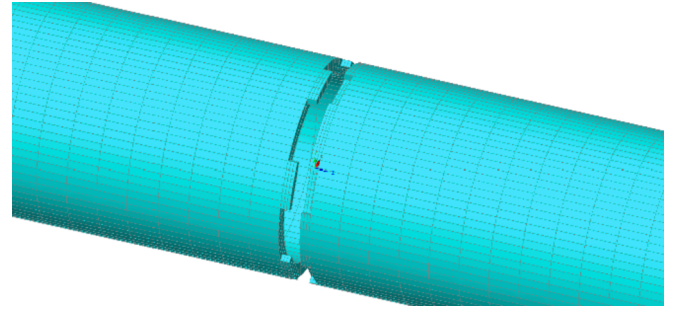
Fig. 8. FE mesh of shear keys applied in the model.
