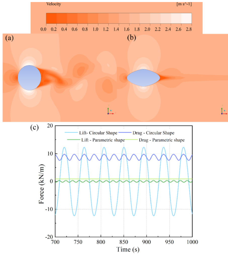
Fig. 14. (a) Instantaneous flow velocity contour for the circular shape; (b) Sequential flow velocity contour for the parametric shape; (c) Drag and lift time-history for the two shapes at V = 1.5 \text{ m/s} .
