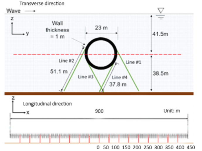
Fig. 1. 2D schematic views of the entire system for the validation case [31].
