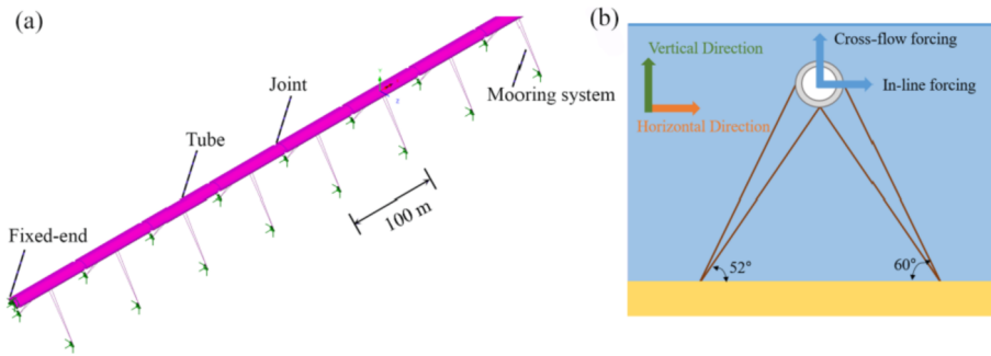
Fig. 11. The SFT model; (a) Coupled tube-joint-mooring system FEM model (Part of the model); (b) Mooring lines arrangement.
