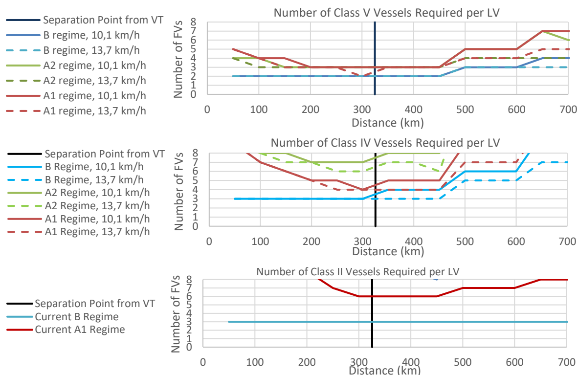
Figure 15: Number of Required Vessels per LV
