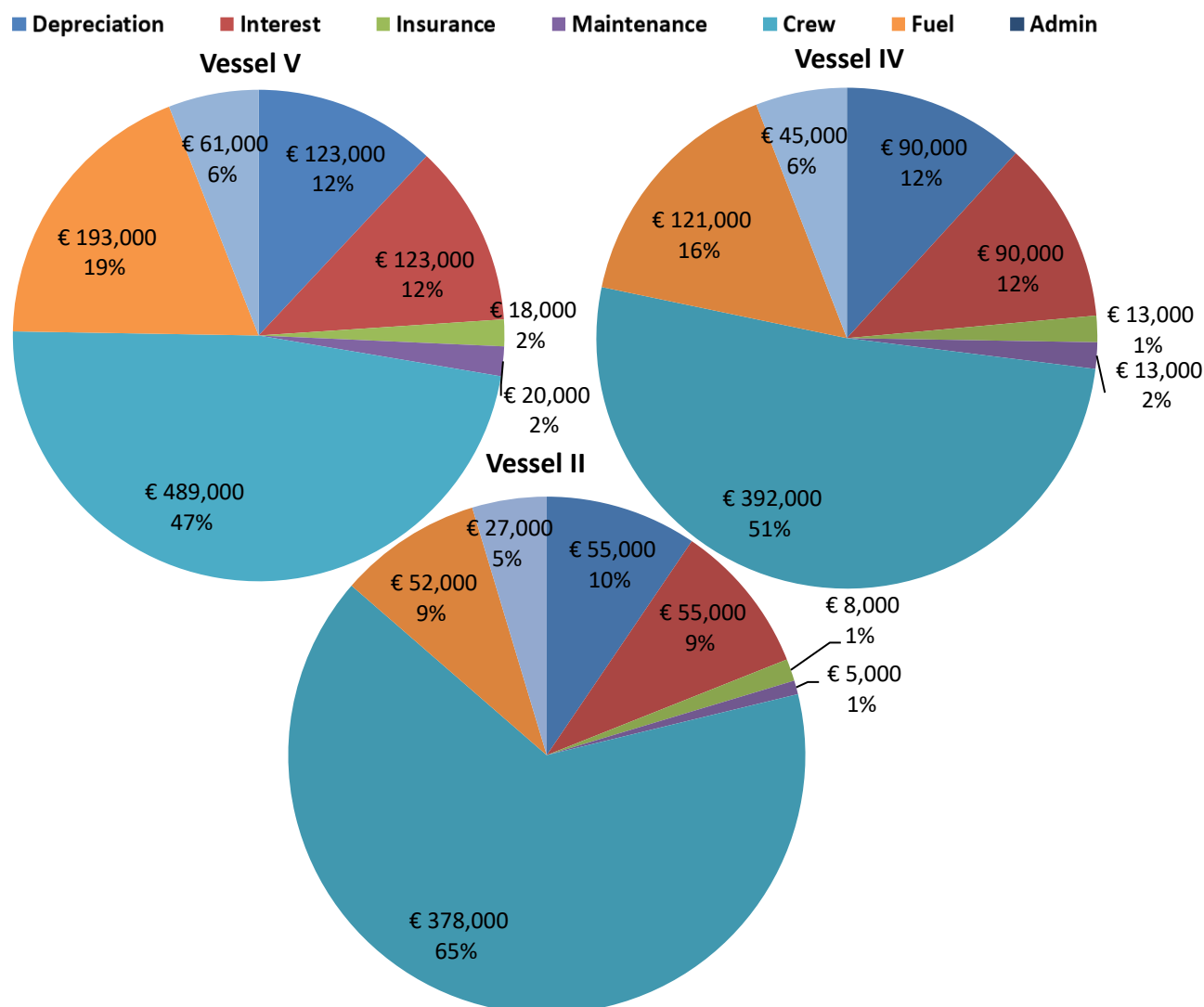
Figure 3: Cost Breakdown under B Operating Regime
