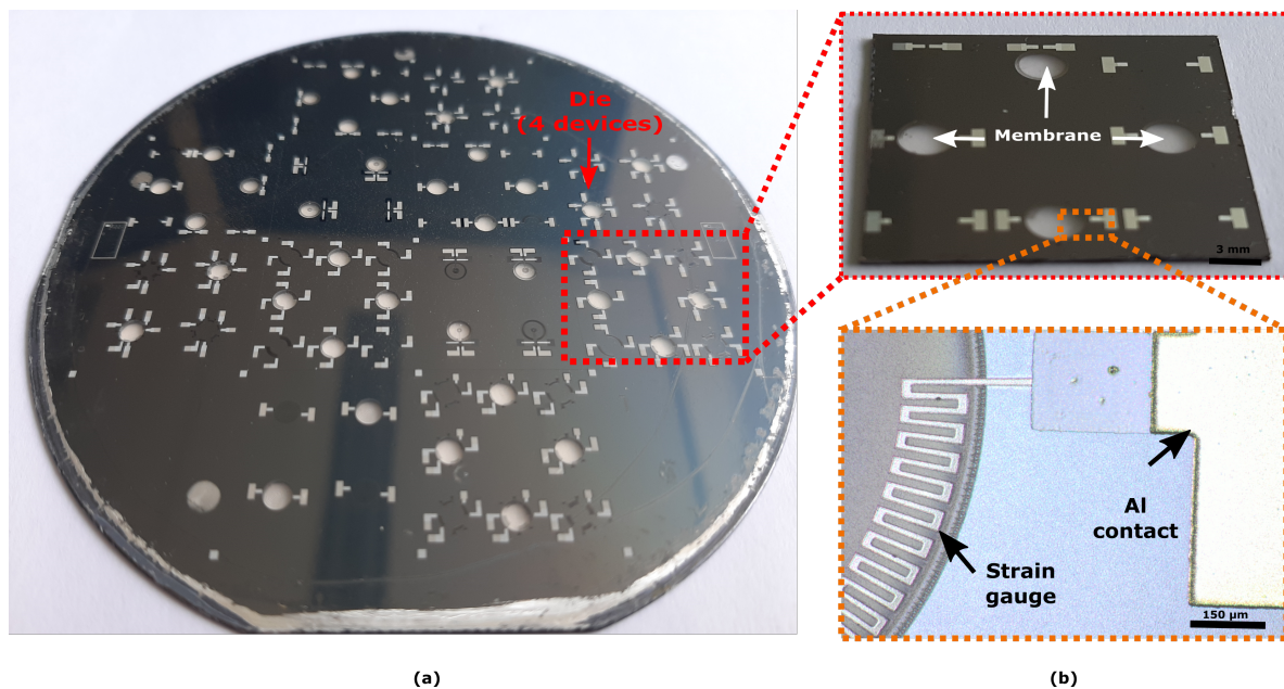
Figure 6. (a) A completed wafer containing 36 membranes equipped with strain gauges. (b) An optical image of a die containing four devices ( top ) and a close-up of the released membranes with Ti gauges ( bottom ). Scale bars: 150 μm ( bottom ), 3 mm ( top ).
