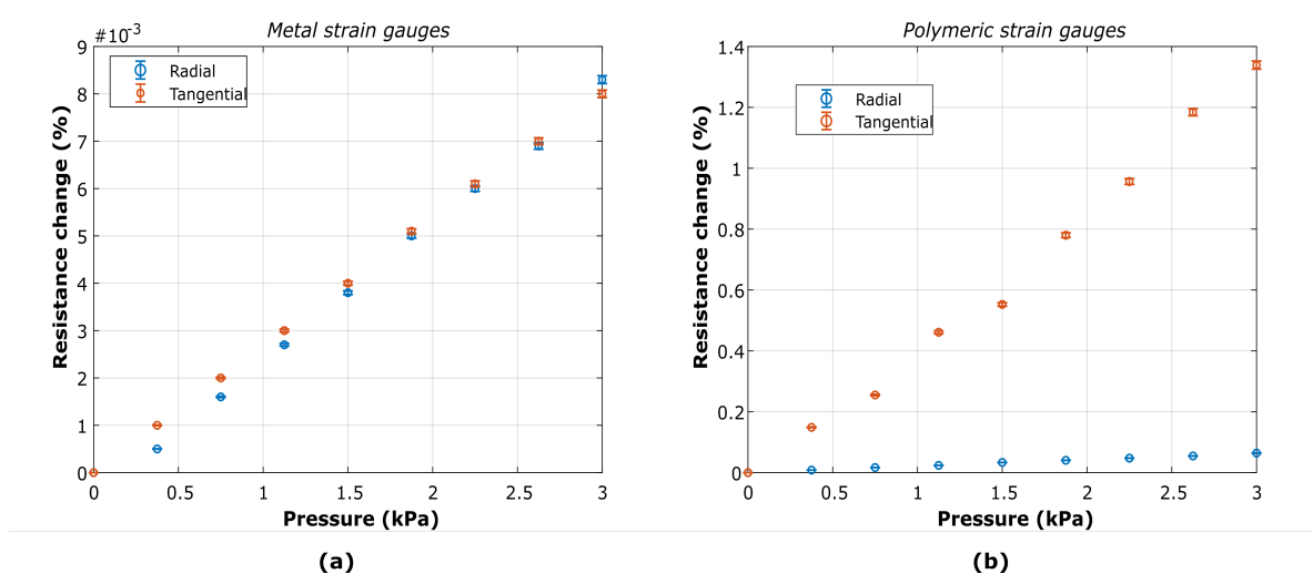
Figure 8. Stationary measurements of resistance change for radial and tangential strain gauges made of (a) titanium (Ti) and (b) PEDOT:PSS. Error bar: 5%.
