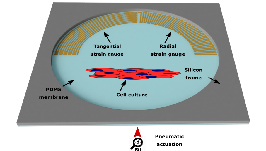
Figure 1. The architecture of the device investigated for stress sensing in a microfabricated PDMS-based OOC platform: Tangential and radial microstructures (strain gauges) on PDMS membranes suspended from a holding silicon frame. The membrane is pneumatically actuated to provide the stretching to a cell culture on its surface.
