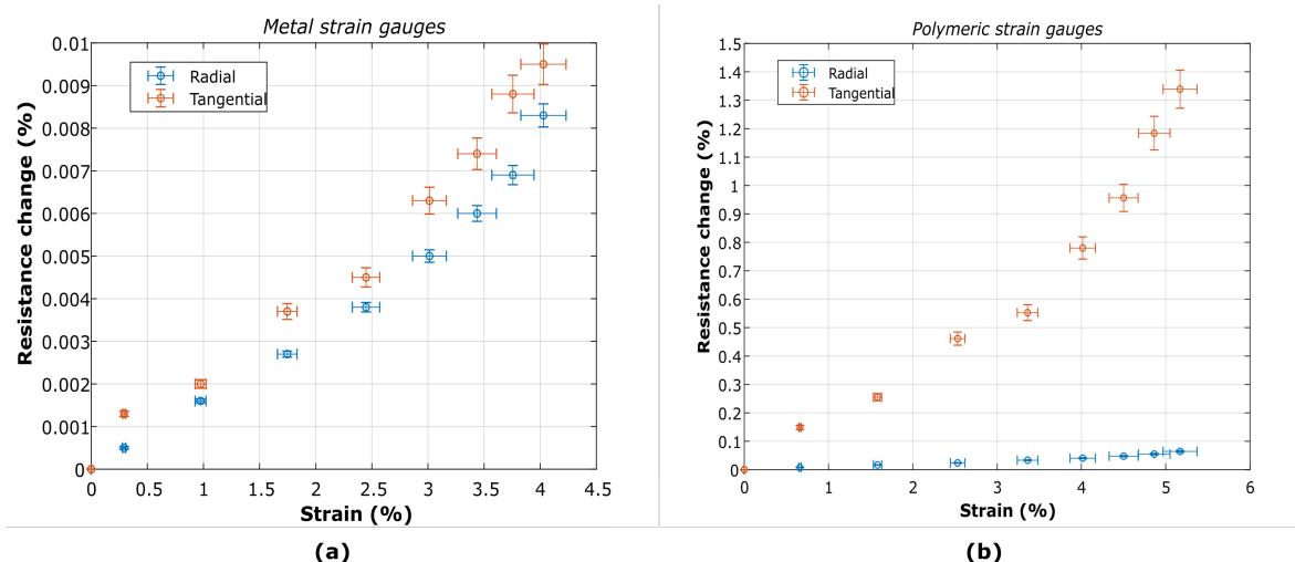
Figure 10. Resistance change as function of the strain on the membrane for radial and tangential strain gauges made of (a) titanium (Ti) and (b) PEDOT:PSS.
