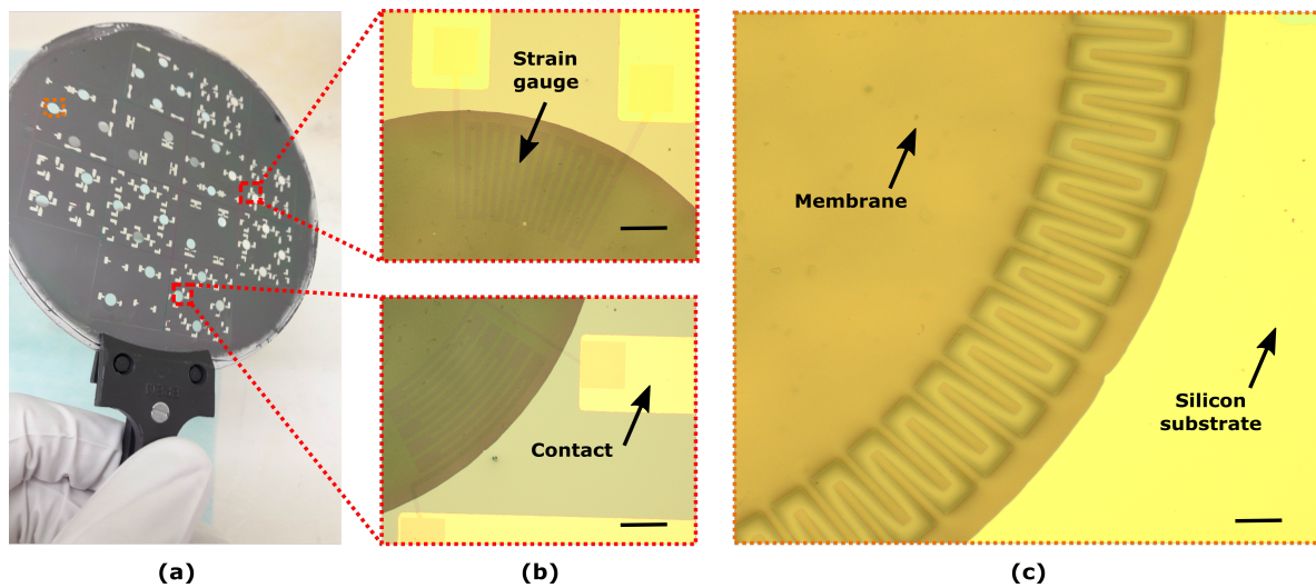
Figure 7. (a) A completed wafer containing 36 membranes equipped with polymeric strain gauges. (b) Optical images of radial (top) and tangential (bottom) polymeric strain gauges embedded in 10 \mu\text{m} -thick PDMS. (c) A zoom-in perspective illustrating the polymeric strain gauges integrated into the PDMS membranes. Scale bar: 100 \mu\text{m} .
