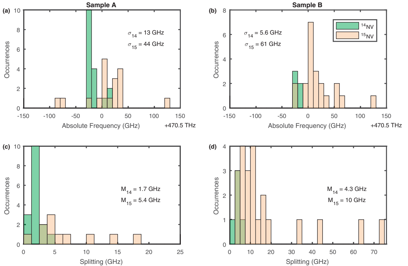
FIG. 4. Strain analysis. (a), (b) The distribution of axial strain (measured by absolute average ZPL frequency) in NVs acquired from analysis of sample A (a) and sample B (b). The ^{15}\text{NV} ZPLs exhibit a larger spread in axial strain (standard deviation, \sigma ) than the ^{14}\text{NV} ZPLs. (c), (d) The distribution of transverse strain (measured by half the splitting between E_x and E_y frequencies) in NV centers of sample A (c) and sample B (d). The ^{15}\text{NV} ZPLs show a greater median splitting ( M ) in both samples.
