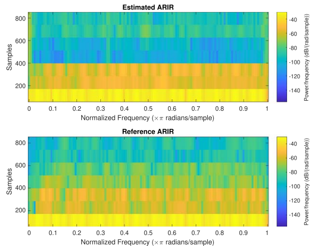
Fig. 6. The spectrogram of an estimated third-order ARIR example with CNN.
