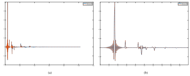
Fig. 8. An estimated first-order ARIR example in the time domain with VCAE. (a) Full signal, (b) the first 200 samples.
