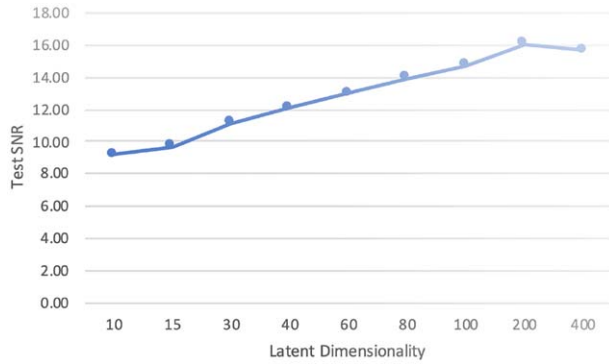
Fig. 7. SNR of estimated ARIR under different dimensionality.
