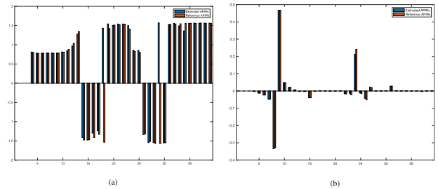
Fig. 10. Reflection analysis of an estimated first-order ARIR example with VCAE. (a) Azimuth of the sound intensity of each time frame in early reflections, (b) elevation of the sound intensity of each time frame in early reflections.
