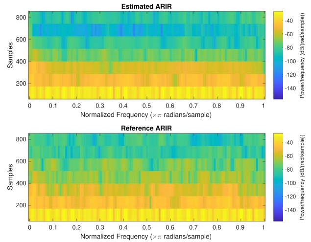
Fig. 9. The spectrogram of an estimated first-order ARIR example with VCAE.
