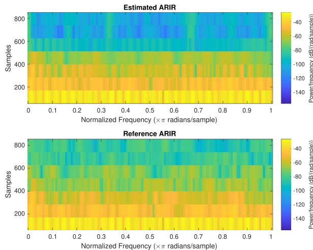
Fig. 3. The spectrogram of an estimated first-order ARIR example with CNN.
