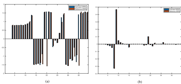
Fig. 4. Reflection analysis of an estimated first-order ARIR example with CNN. (a) Azimuth of the sound intensity of each time frame in early reflections, (b) elevation of the sound intensity of each time frame in early reflections.
