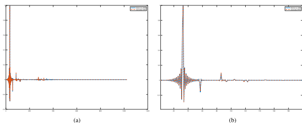
Fig. 5. An estimated third-order ARIR example in the time domain with CNN. (a) Full signal, (b) the first 200 samples.
