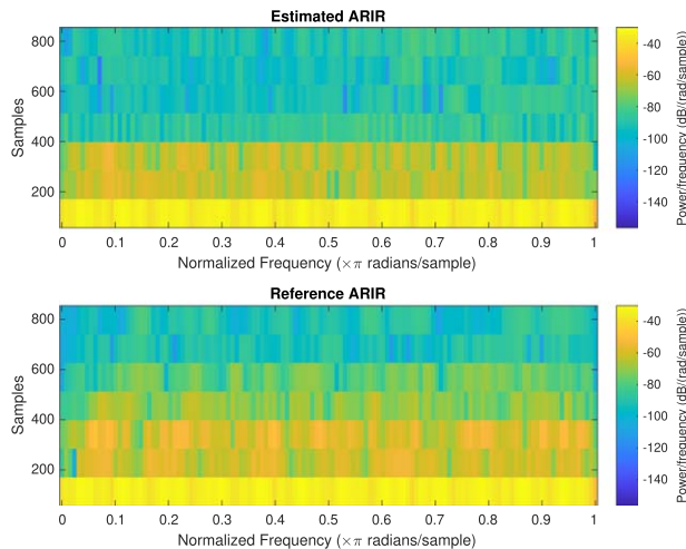
Fig. 12. The spectrogram of an estimated third-order ARIR example with VCAE.
