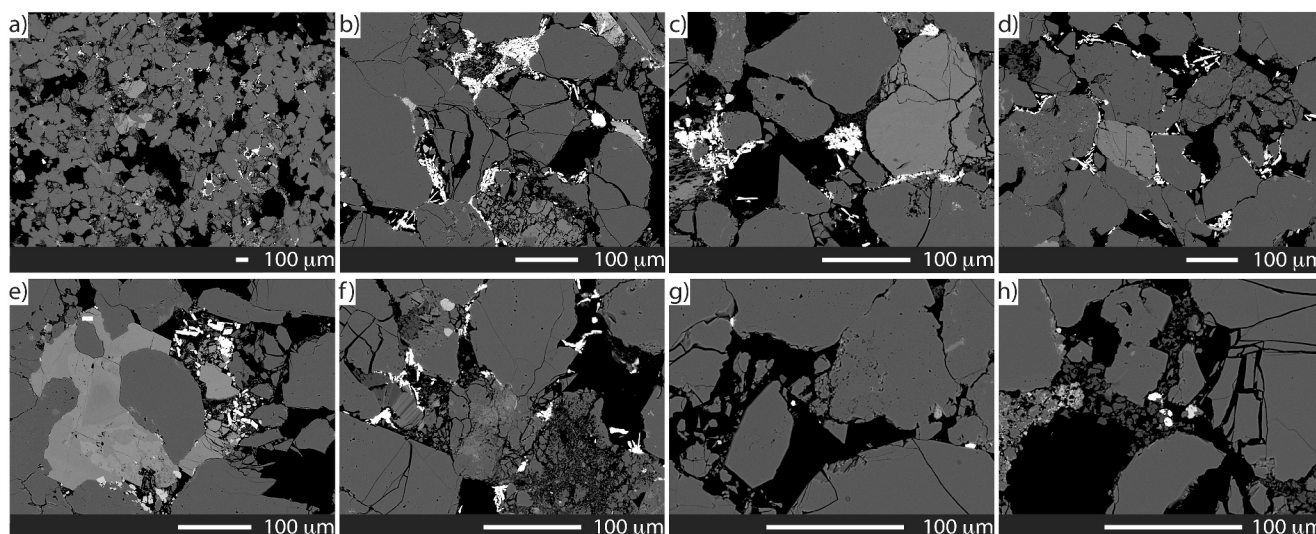
Figure 5. Backscattered Electron (BSE) images of a thin section from Experiment 2, captured at magnifications between 40× and 500×. Panels (a–f) show images from the precipitation boundary, while (g, h) depict areas inside the precipitation curtain (i.e., the region flooded by the \text{BaCl}_2 solution). The specific locations of these images correspond to the XRCT axial cross section shown in Figure S3 in Supporting Information S1. Here, barite is represented by the bright white regions.
