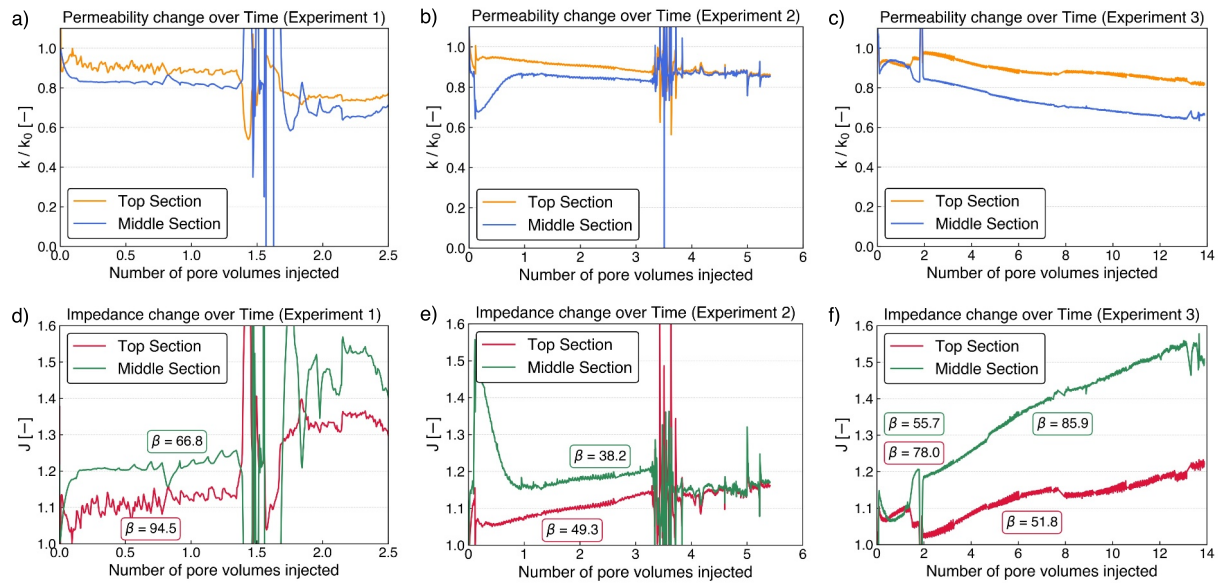
Figure 3. Temporal evolution of normalized permeability, k/k_0 (Panels a–c) and impedance index, J (Panels d–f), for the top and middle sections of the core sample, calculated from the differential pressures recorded by the sensors dP1 and dP2, respectively.
