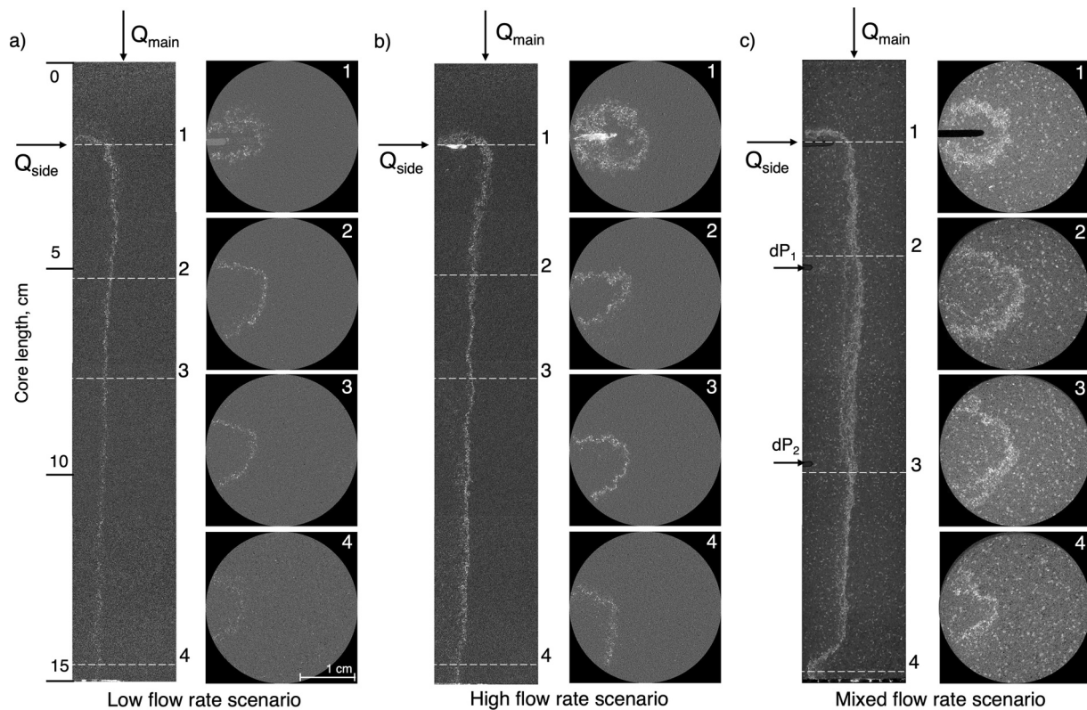
Figure 4. Coronal (vertical) and axial (horizontal) cross sections of XRCT images showing the barite precipitation profiles for (a) Experiment 1, (b) Experiment 2, and (c) Experiment 3. The dashed lines (1–4) indicate the locations of the axial cross sections along the core. Precipitated barite is visible as bright spots in the images. The images in (a, b) were generated by subtracting the registered pre- and post-experiment scans, while the images in (c) show the raw post-experiment scan, which contains natural rock inclusions.
