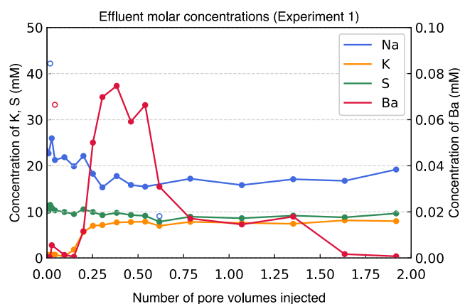
Figure 7. Temporal variation of cation molar concentrations in collected effluent as determined by inductively coupled plasma mass spectrometry. Empty data points represent outliers, based on the chemically reasonable Na/S ratio of the \text{Na}_2\text{SO}_4 solution.
