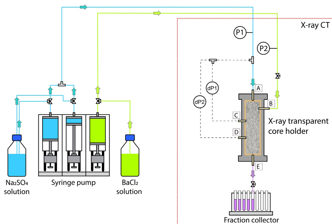
Figure 1. Schematic drawing of the core-flooding system, where two incompatible fluids ( \text{Na}_2\text{SO}_4 and \text{BaCl}_2 ) are injected simultaneously into a core holder positioned inside the X-ray micro-CT scanner (injection points A and B, respectively). The effluent is continuously sampled at the outlet (E) using a fraction collector. Pressure sensors P1 and P2 measure absolute pressure, and differential pressure sensors dP1 and dP2 register pressure drop across the top (C) and middle (D) sections of the core, respectively.
