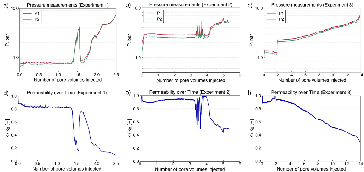
Figure 2. Evolution of pressure and normalized bulk permeability for the three experiments. Panels (a–c) demonstrate pressure changes over time, where P1 represents the inlet pressure of the main axial flow (top injection) and P2 corresponds to the inlet pressure of the side injection. Panels (d–f) show normalized permeability, k/k_0 (i.e., the reciprocal of the impedance index) for each respective core sample. The sharp fluctuations observed in Experiments 1 and 2 are attributed to temporary blockages in the outlet tubing.
