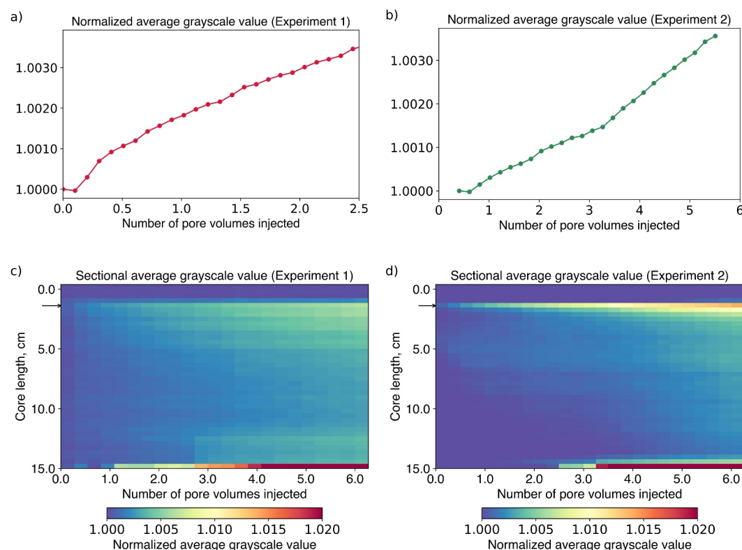
Figure 6. Temporal evolution of the normalized grayscale value for Experiments 1 and 2, calculated from the in situ 2D radiographs. Panels (a, b) show the temporal evolution of the normalized average grayscale values for the entire core sample, while Panels (c, d) present the spatial-temporal evolution of the normalized average grayscale values across multiple sections along the core length. All values were normalized against a baseline radiograph taken prior to the experiments. Values greater than 1 indicate an increase in mineral density compared to the baseline image, serving as a proxy for the increased barite content in the rock core.
