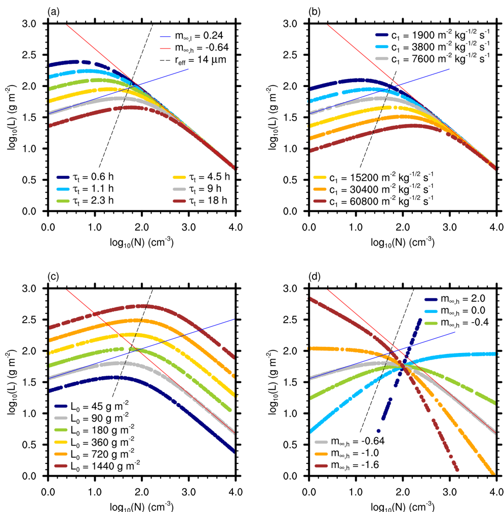
Figure 2. L after 7 d as a function of N for variations in (a) \tau_i , (b) c_1 , (c) L_0 , and (d) m_{\infty,h} (colored dots). The default configuration is differentiated by gray dots. Plots are overlaid with m_{\infty,l} = 0.24 and m_{\infty,h} = -0.64 (blue and red lines) and the 14\mu\text{m} cloud top effective droplet radius (dashed black line).
