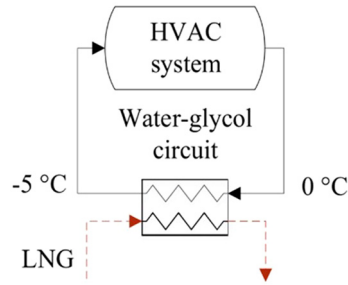
Figure 5.16 Scheme of proposed system to recover the wasted cold for marine HVAC [32].
