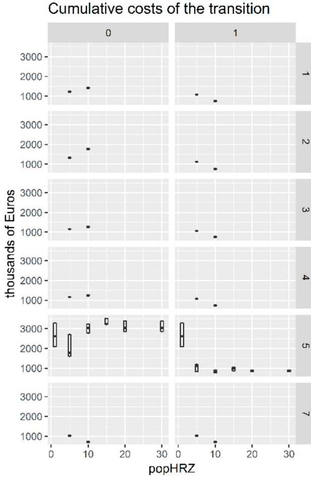
Figure 3.6: Cumulative costs of the transition (gas-free-subset). Each plot displays results from simulation runs with a unique combination of popACCI (grey labels on top of each column) and popORI (grey labels to the right of each row). In each plot, a boxplot is displayed for simulation runs with the same popHRZ, e.g., the plot in the top right corner displays simulation runs in which popACCI = 1.00 and popORI = 1, the first boxplot corresponds to popHRZ = 5, and the second one, to popHRZ = 10.
