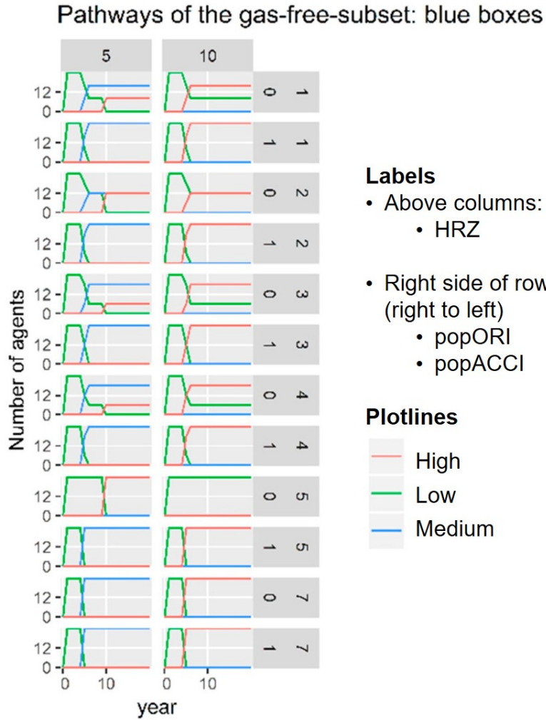
Figure 3.10: Pathways of the gas-free-subset when \text{popHRZ} = 5 or 10 , \text{dgp} = 0.04 , and \text{dep} = -0.04 , classified by \text{popHRZ} (grey labels on top of each column) and a unique combination of \text{popORI} and \text{popACCI} (labels on the right side of each row). Each line plot shows the number of dwellings with each insulation level over time. These plots are a zoom-in on the content of the blue frames in Figure 3.8. Legend is adapted with respect to Nava Guerrero et al. [2019].
