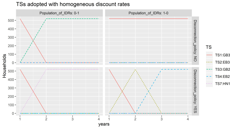
Figure 4.3: TSs adopted in the neighbourhood when households had homogeneous discount rates. The left column represents populations in which all households had \rho_{market} (0–1), and the right, \rho_{bnd} (1–0).
