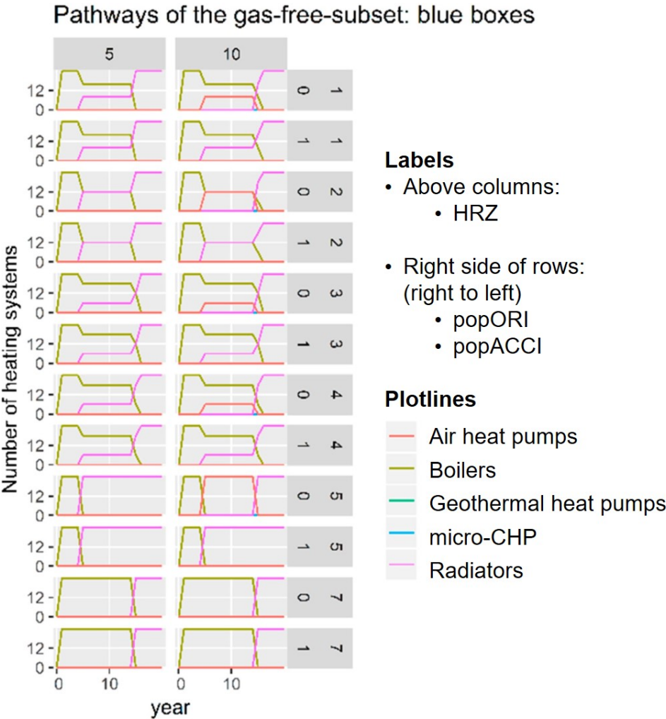
Figure 3.9: Pathways of the gas-free-subset when \text{popHRZ} = 5 or 10 , \text{dgp} = 0.04 , and \text{dep} = -0.04 , classified by \text{popHRZ} (grey labels on top of each column) and a unique combination of \text{popORI} and \text{popACCI} (labels on the right side of each row). Each line plot shows the number of dwellings with each heating system over time. These plots are a zoom-in on the content of the blue frames in Figure 3.7. Legend is adapted with respect to Nava Guerrero et al. [2019].
