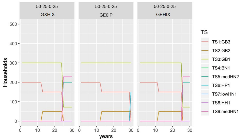
Figure 5.3: TSs of households in partial transitions when HPP=50-25-0-25 per RE.
