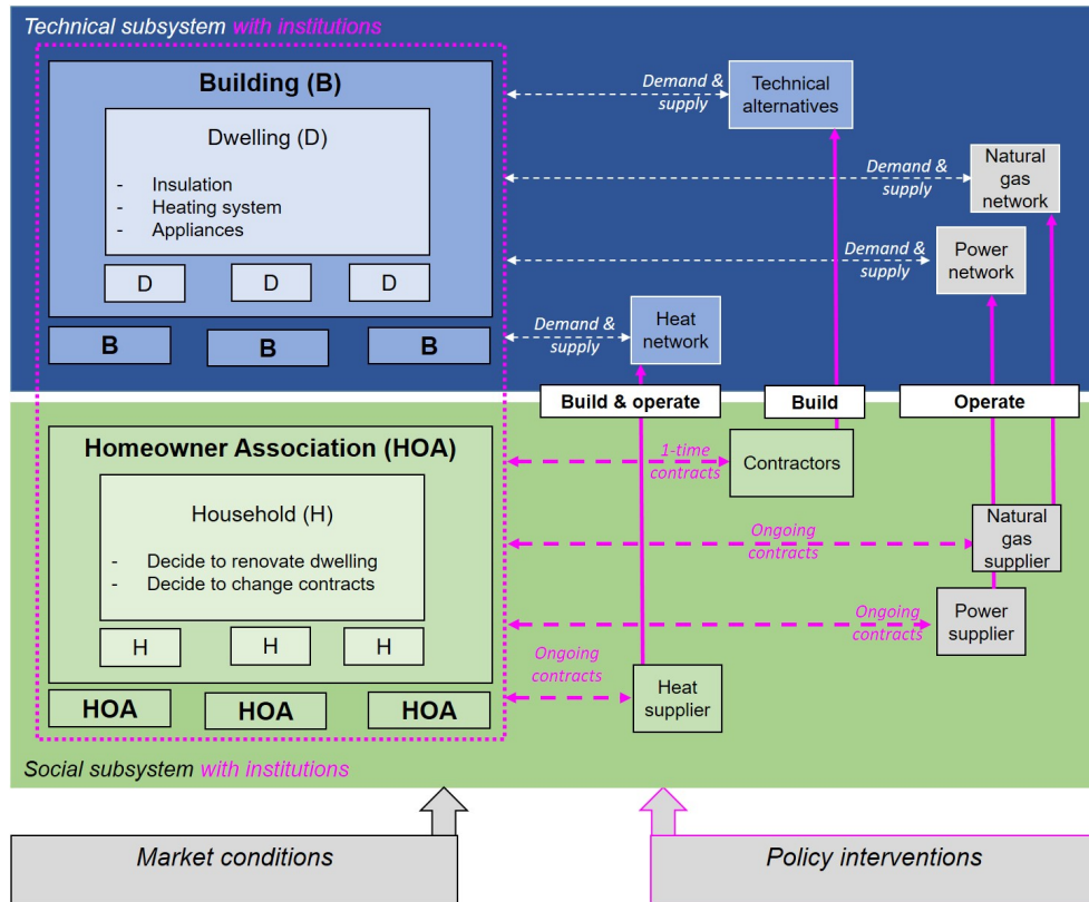
Figure 4.1: Illustration of our view of the problem at the level of one neighbourhood, from the perspective of STS and CAS.
