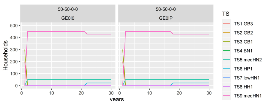
Figure 5.4: TSs of households in full transitions when HPP=50-50-0-0 per RE.
