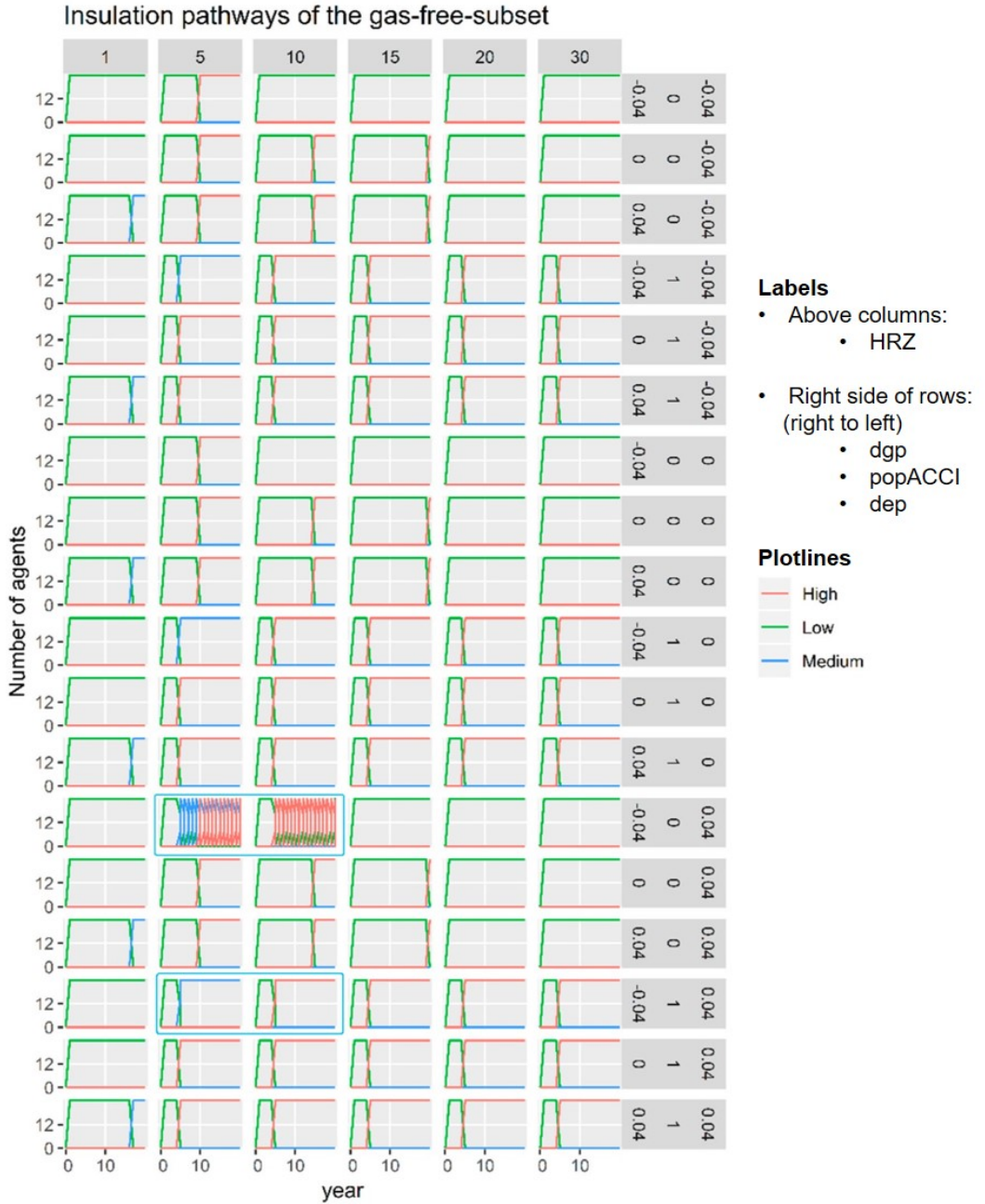
Figure 3.8: Insulation pathways of the gas-free-subset, classified by popHRZ (grey labels on top of each column) and a unique combination of dgp, popACCI, and dep (labels on the right side of each row). Each line plot shows the number of dwellings with each insulation level over time. Blue frames indicate pathways from simulation runs where popORI = 1, 2, 3, 4, 5, or 7. Each plot without a blue frame contains only the pathway for popORI = 5. Legend is adapted with respect to Nava Guerrero et al. [2019].
