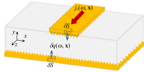
Fig. 11. Microstrip line with rough surface of printed conductors bonded to dielectric substrate with permittivity \epsilon_r . Heat \delta q(\omega, \mathbf{x}) , generated by surface current with density j_c(\omega, \mathbf{x}) of frequency \omega at point \{\mathbf{x}: x, z\} on conductor incremental surface areas \delta S , flows into substrate.
