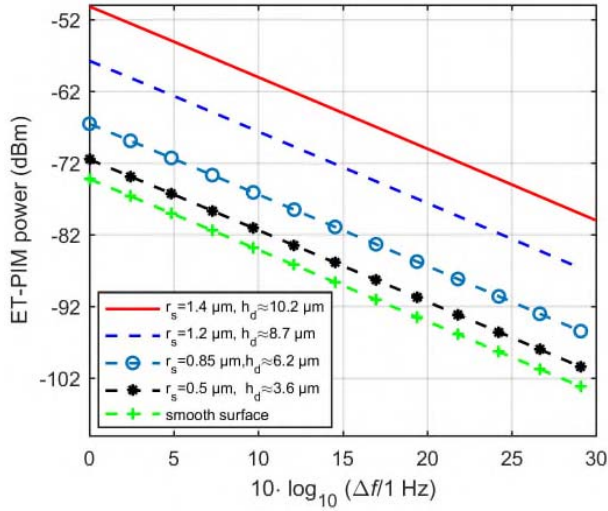
Fig. 4. PIM3 products at 400 MHz in microstrip TLs with copper conductors of various roughness versus carrier frequency offset \Delta f . The microstrip TL parameters are specified in Fig. 3.
