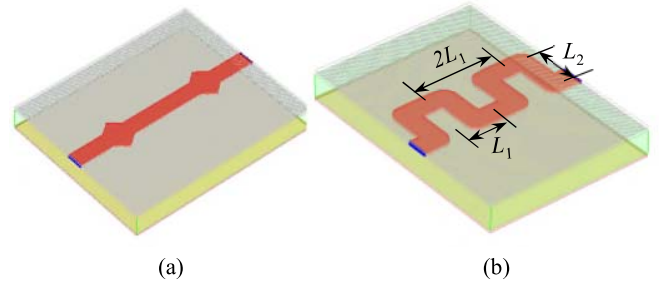
Fig. 8. Microstrip line with (a) periodic rhombus-shaped patches and (b) meandered strip.
