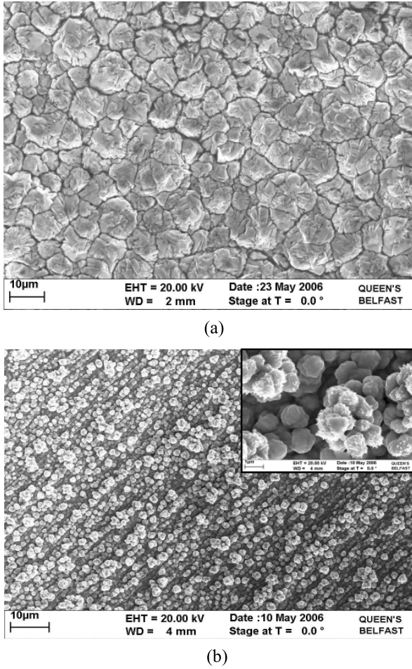
Fig. 1. SEM images of (a) shiny and (b) treated sides of PCB copper cladding. Enlarged image of dendrite clusters is shown in the inset of (b).
