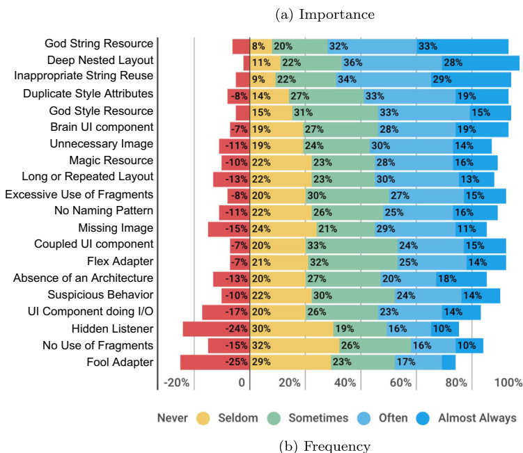
Fig. 3 Frequency and importance of the proposed code smells, according to our participants' perceptions
